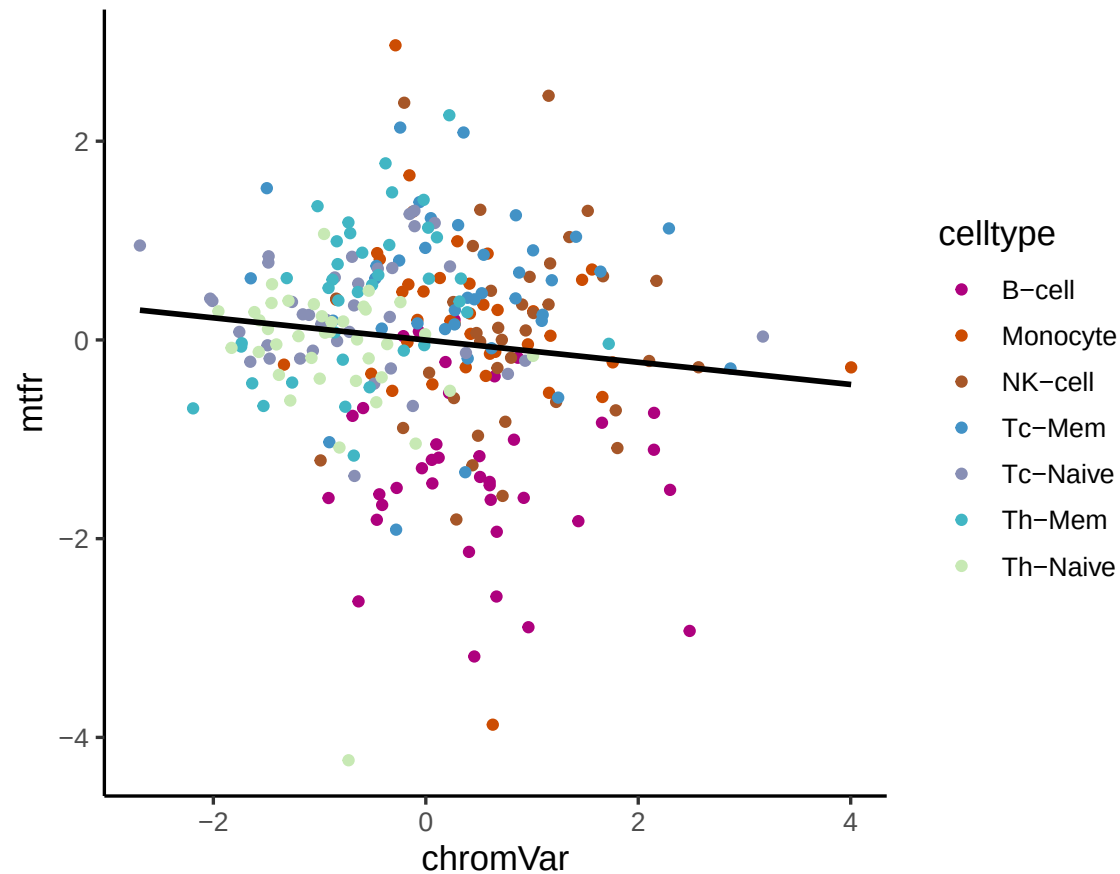
TF Activity Correlation (chromVar vs mtfr) for LHX6
