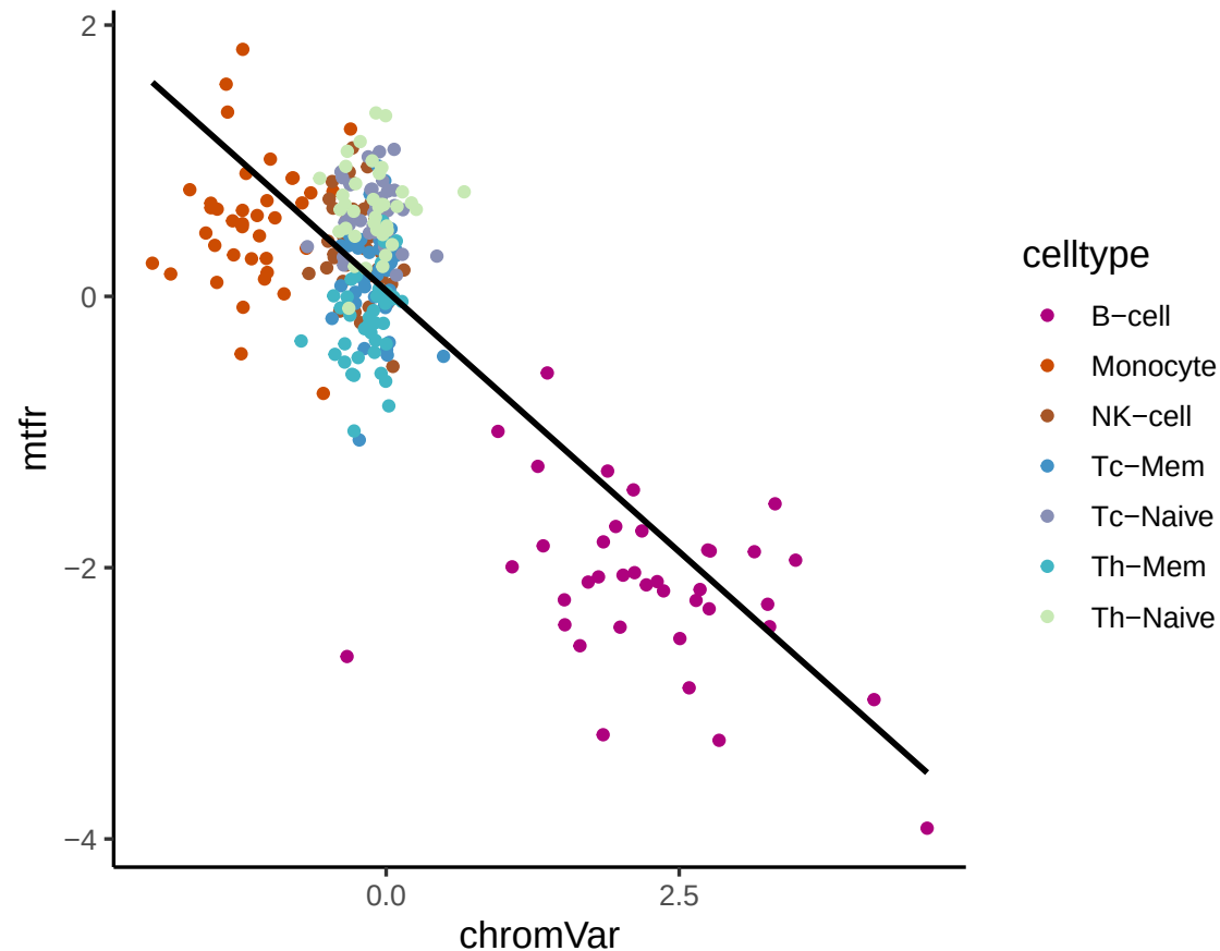
TF Activity Correlation (chromVar vs mtfr) for POU2F2
