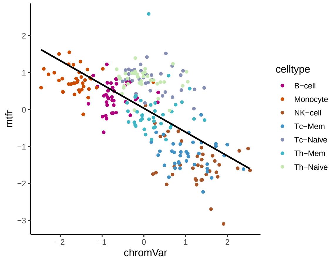
TF Activity Correlation (chromVar vs mtfr) for TBX2
