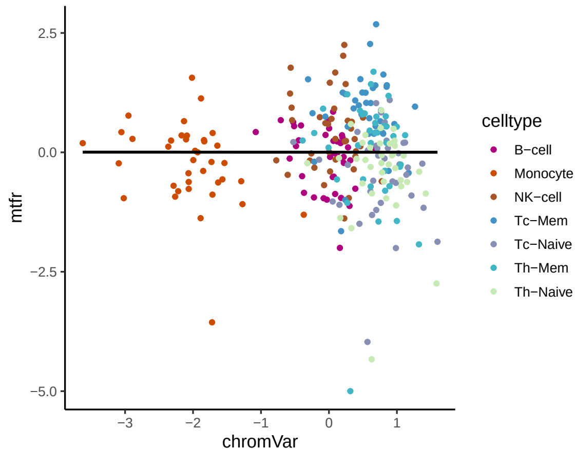
TF Activity Correlation (chromVar vs mtfr) for ZBTB14
