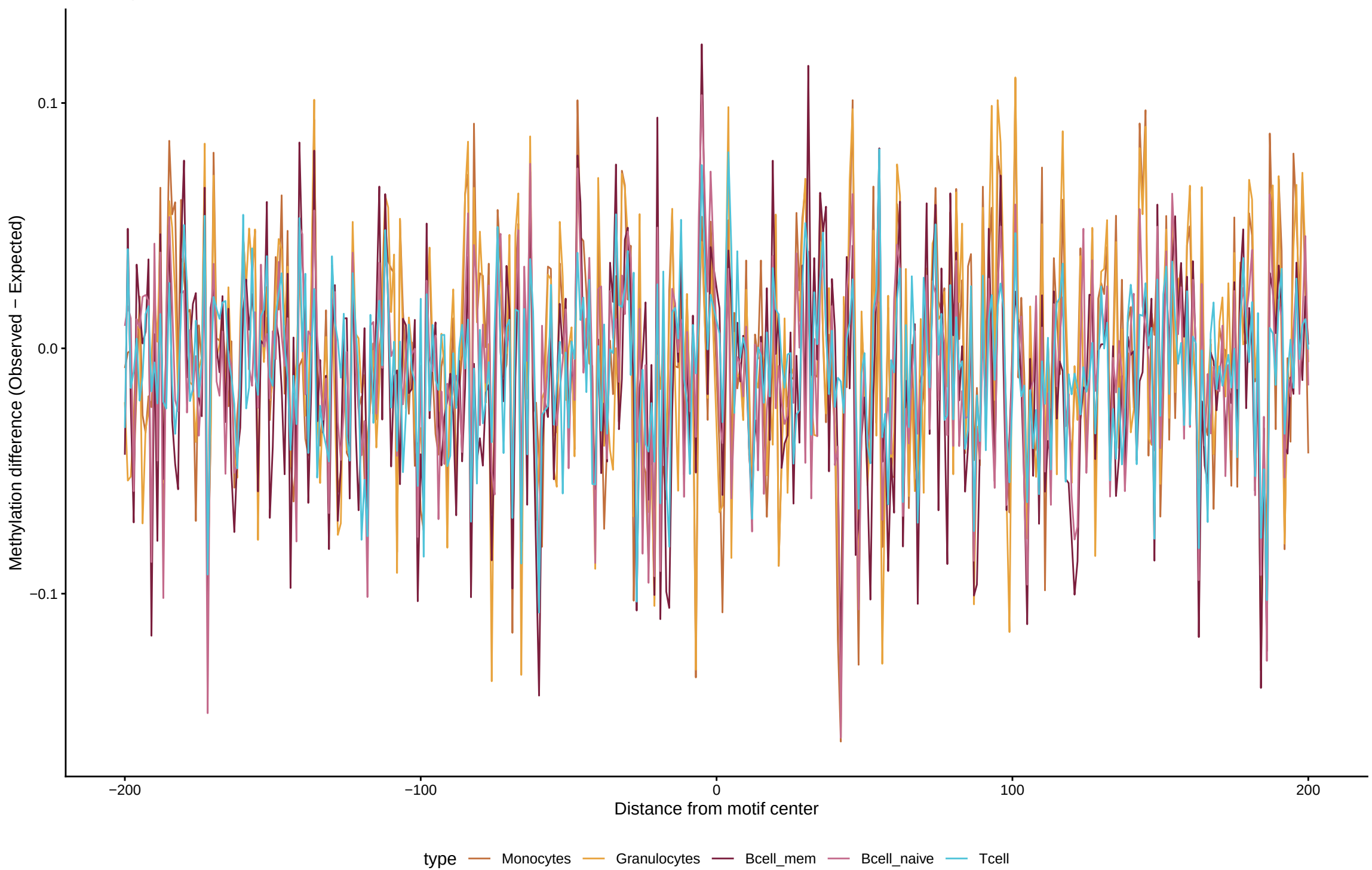
TF footprint difference for BHLHE22
