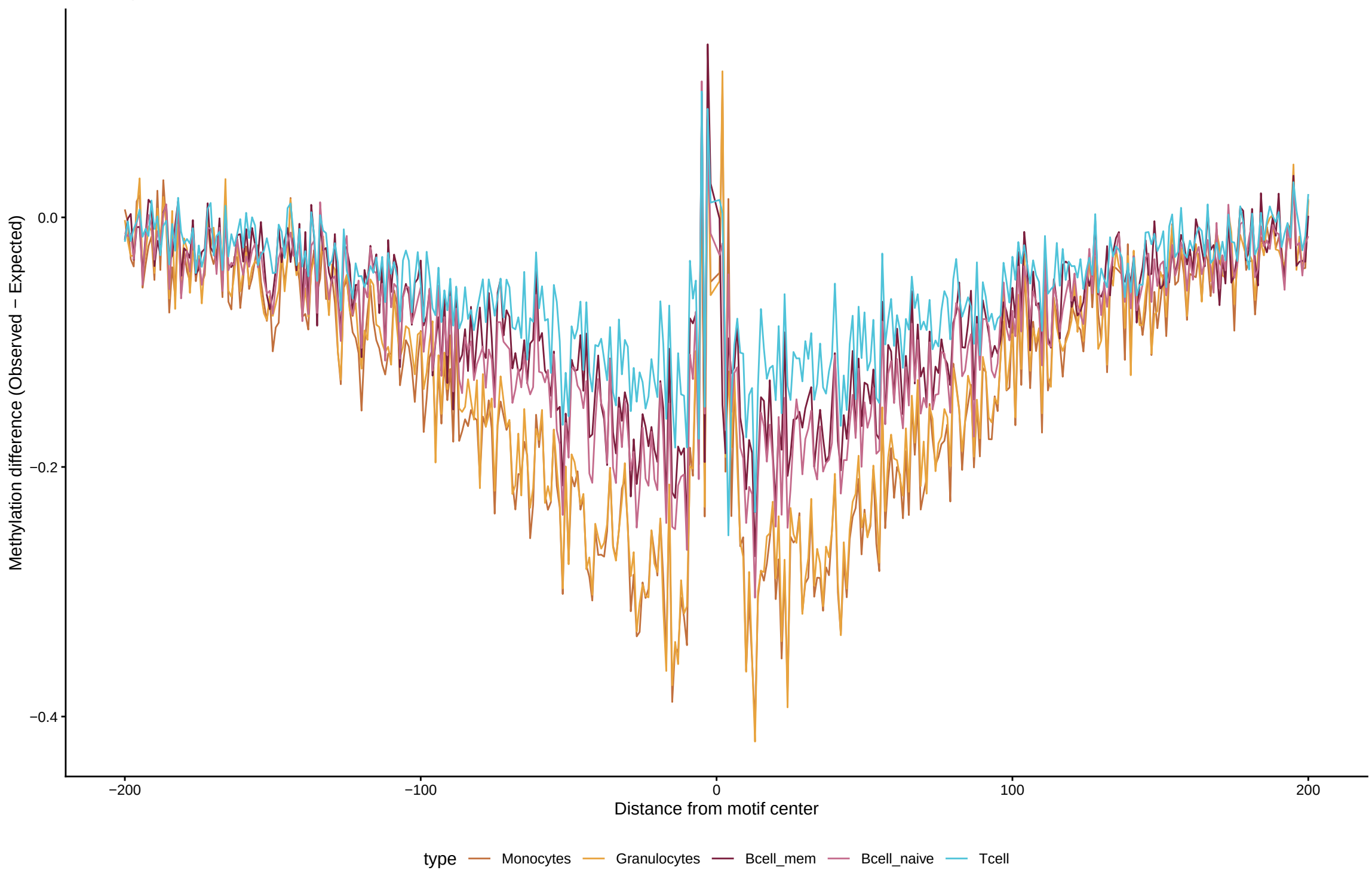
TF footprint difference for ELF5
