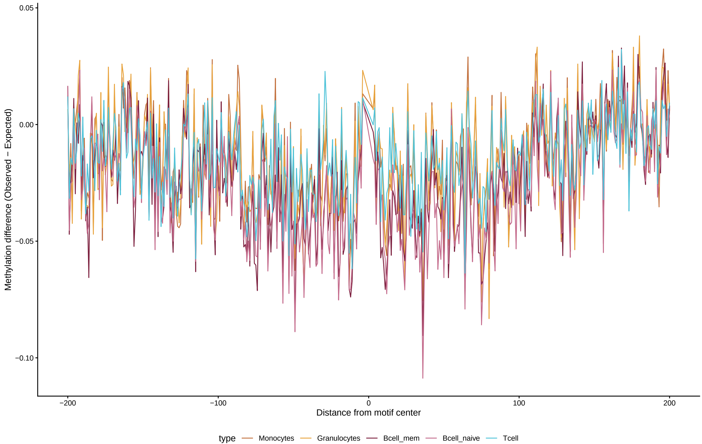
TF footprint difference for NHLH1
