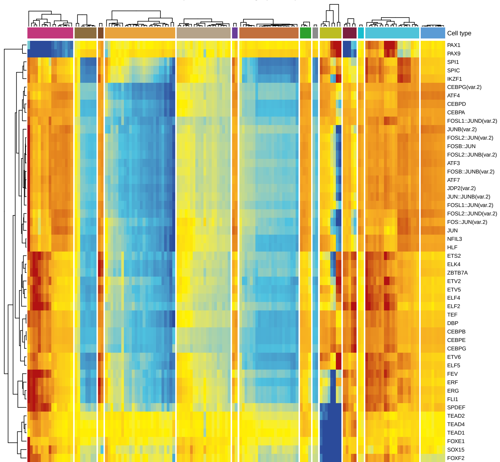
Top 50 differential TFs (jaspar2020)
