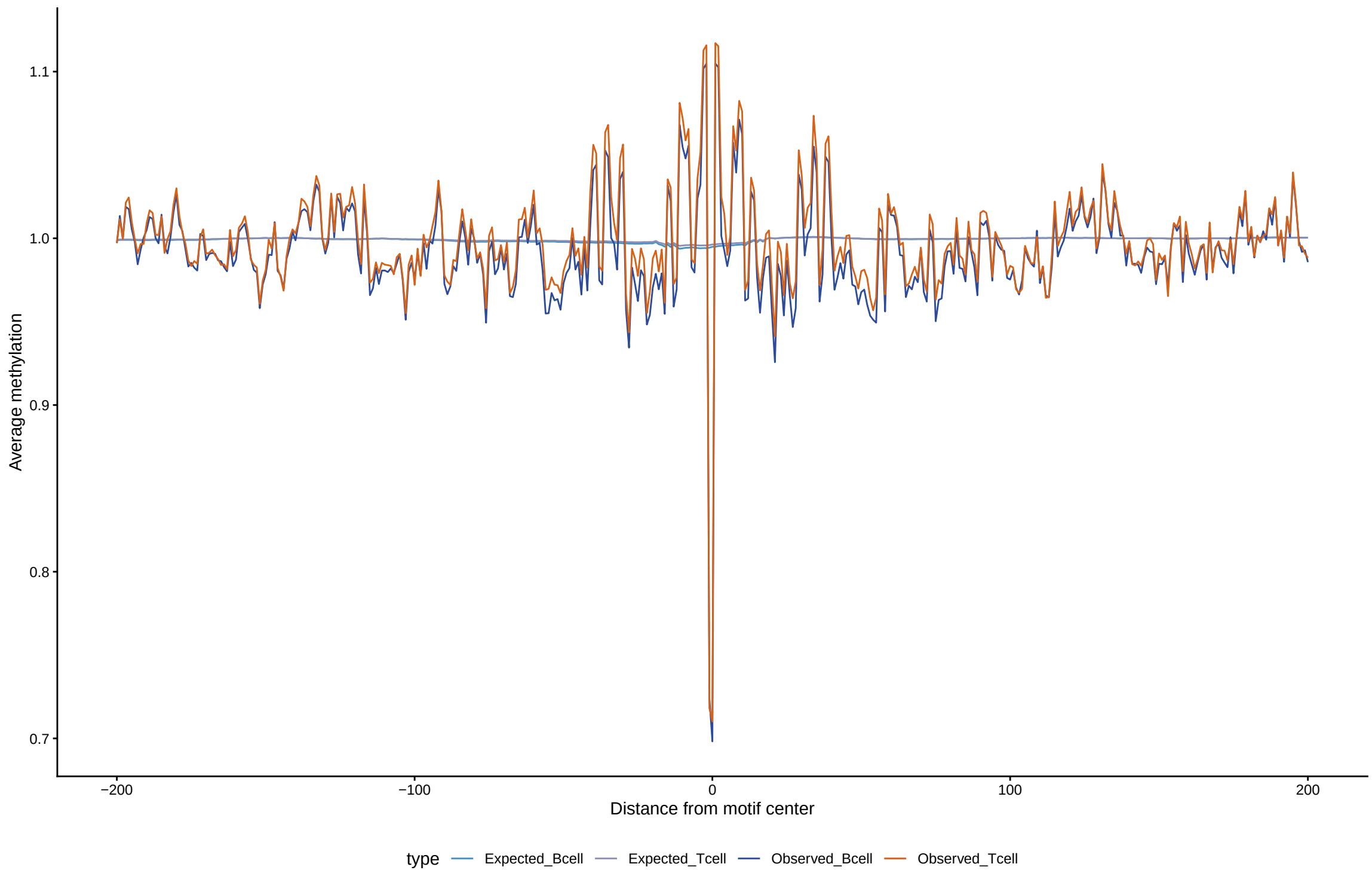
Expected vs observed footprints for PAX5
