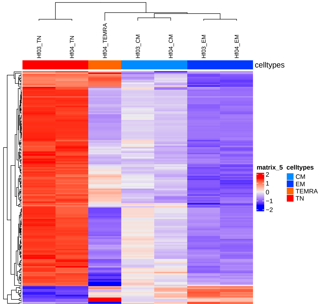
Z-Scores of differential TFs
