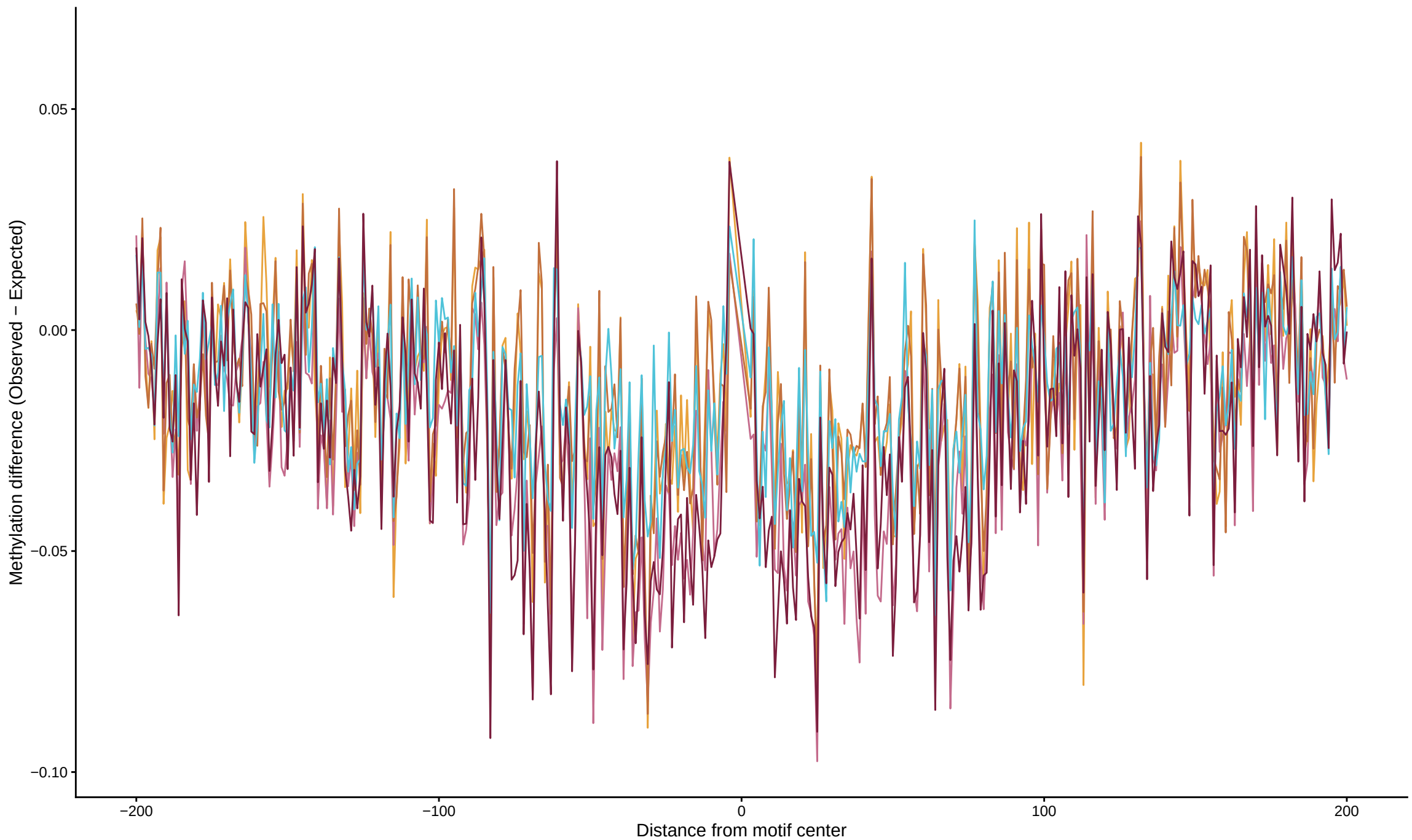
TF footprint difference for ASCL1
