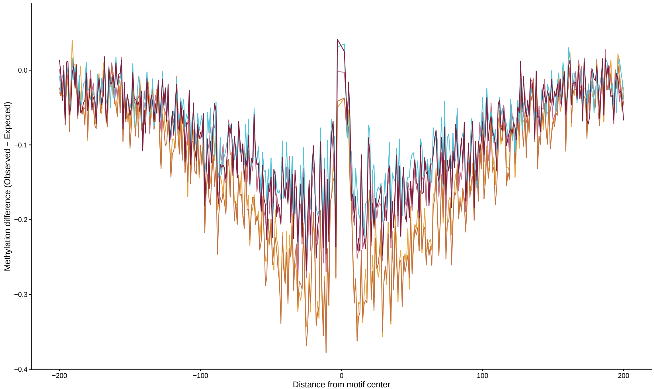
TF footprint difference for ETV5
