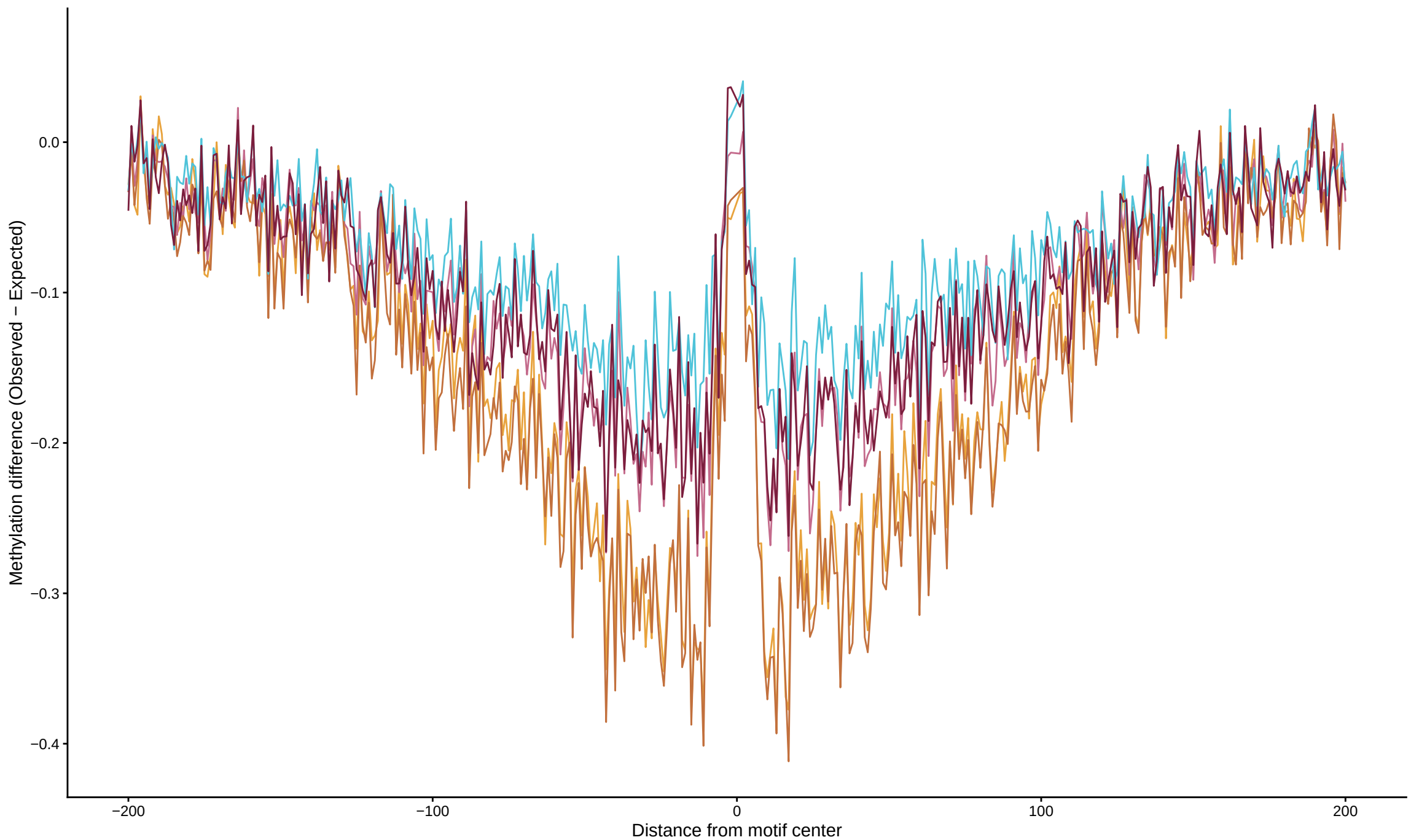
TF footprint difference for ETV6
