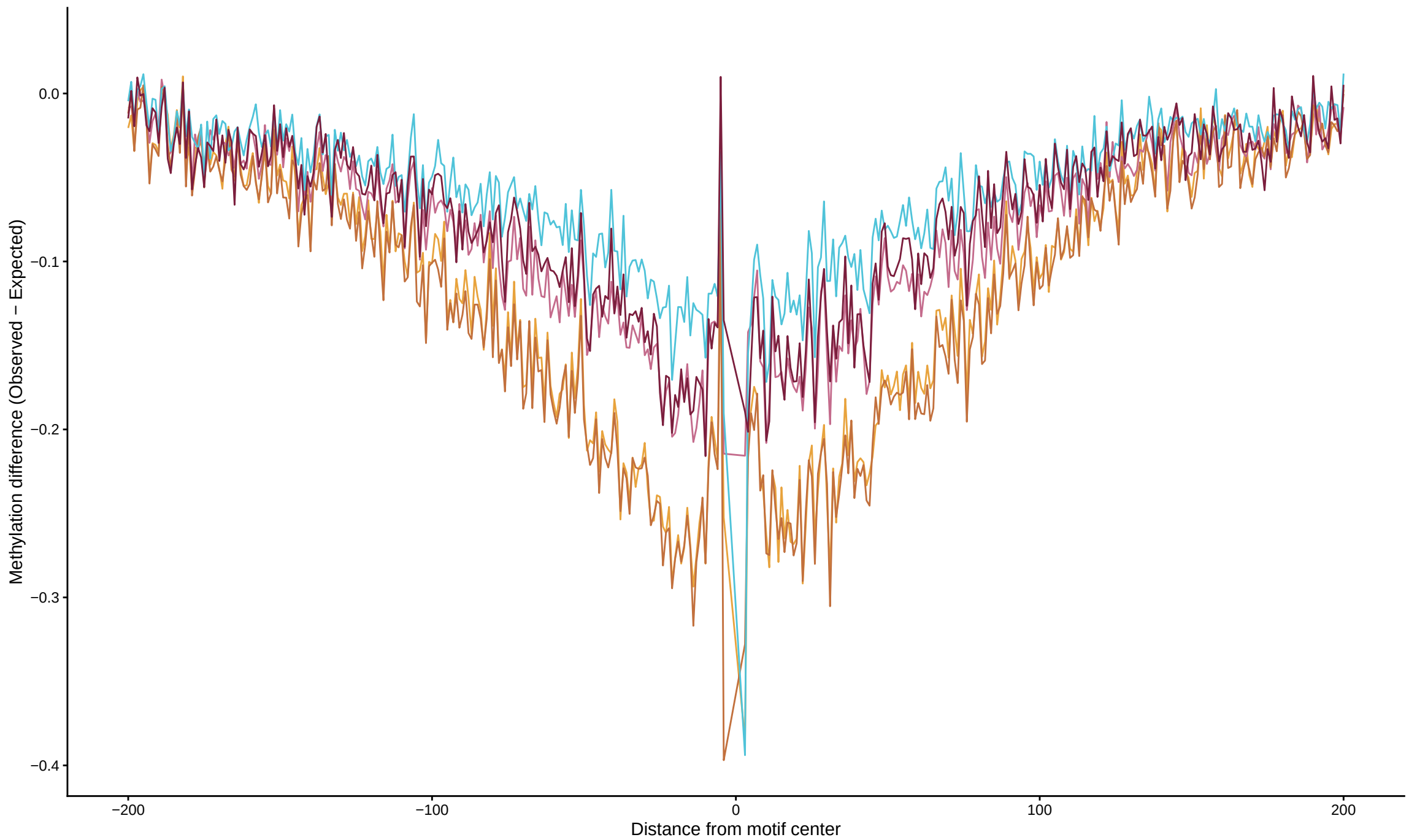
TF footprint difference for IKZF1
