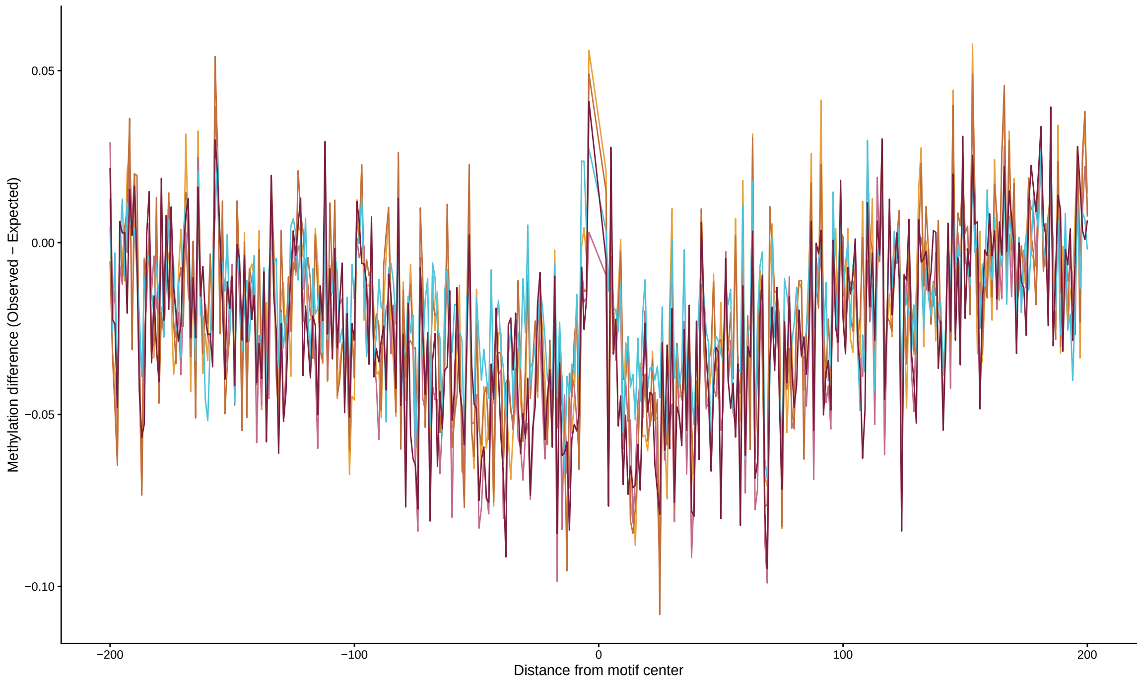
TF footprint difference for MYF5
