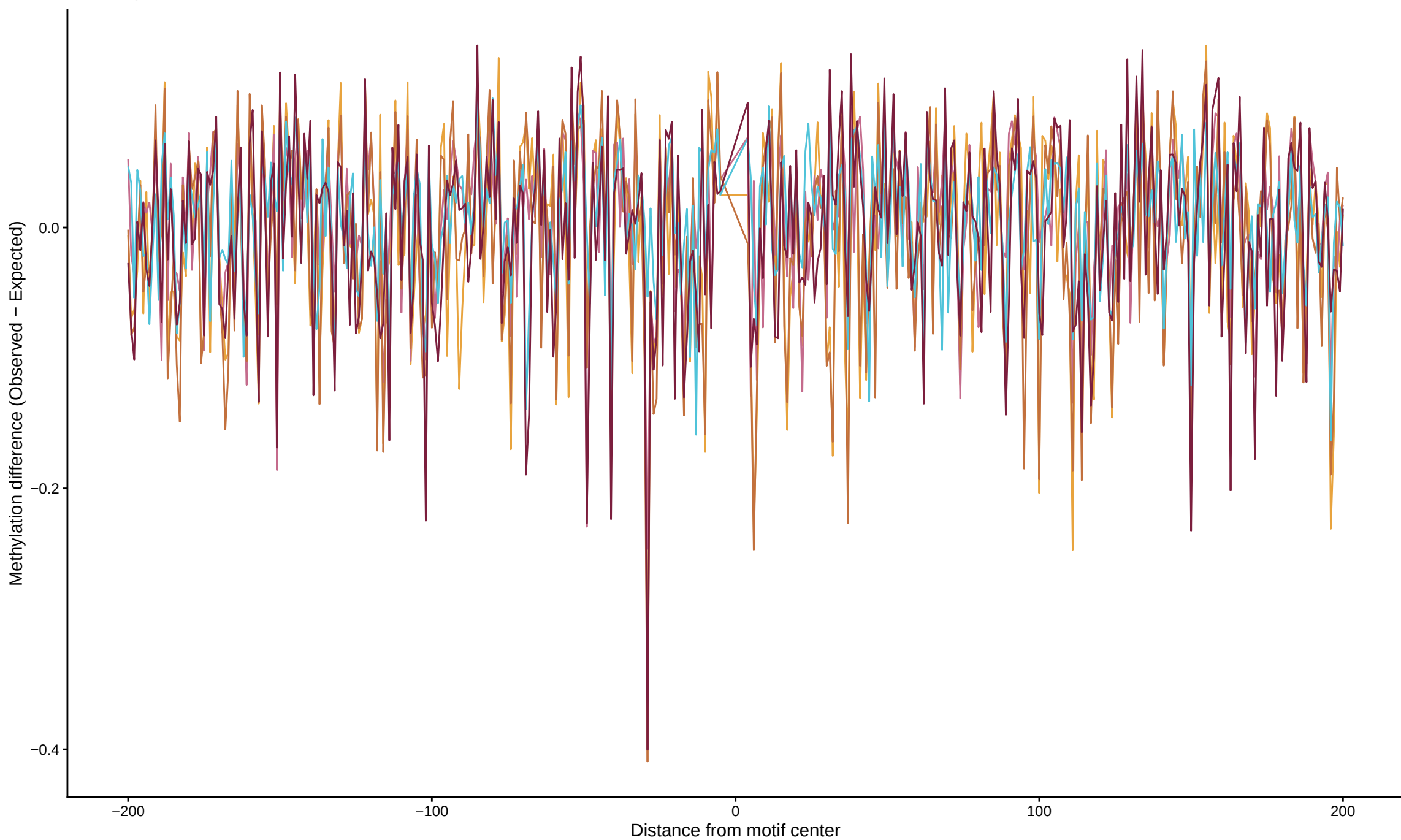
TF footprint difference for PAX4
