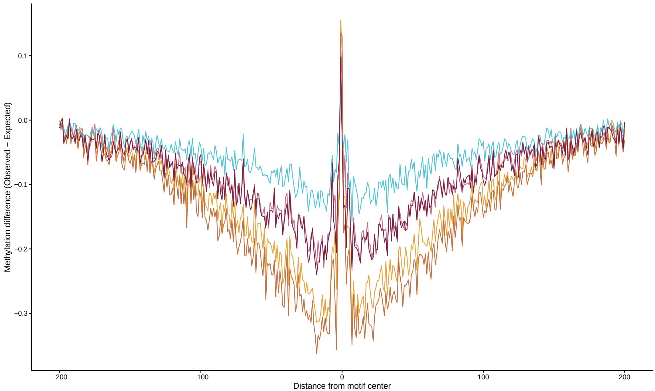
TF footprint difference for SPIB
