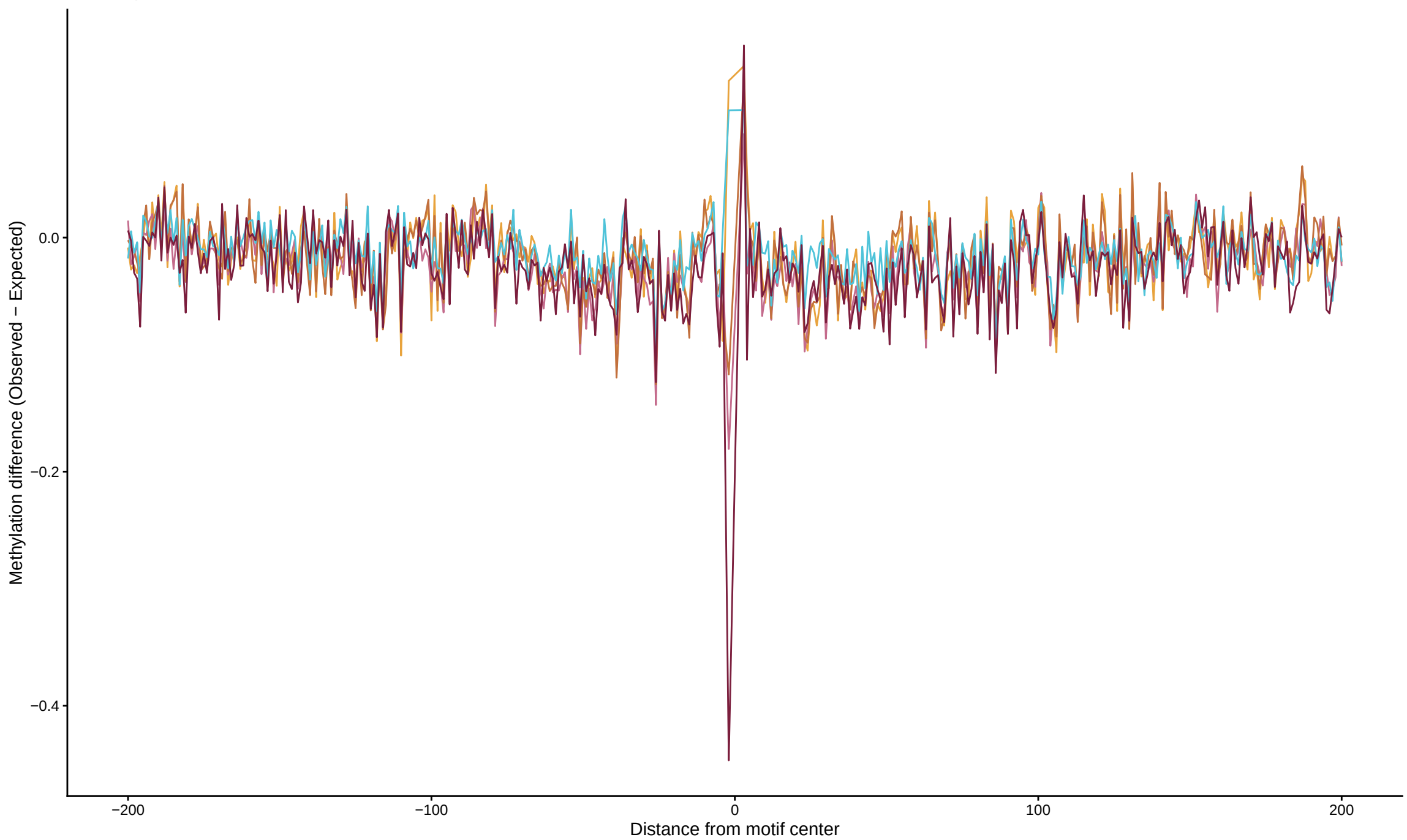
TF footprint difference for TAL1::TCF3
