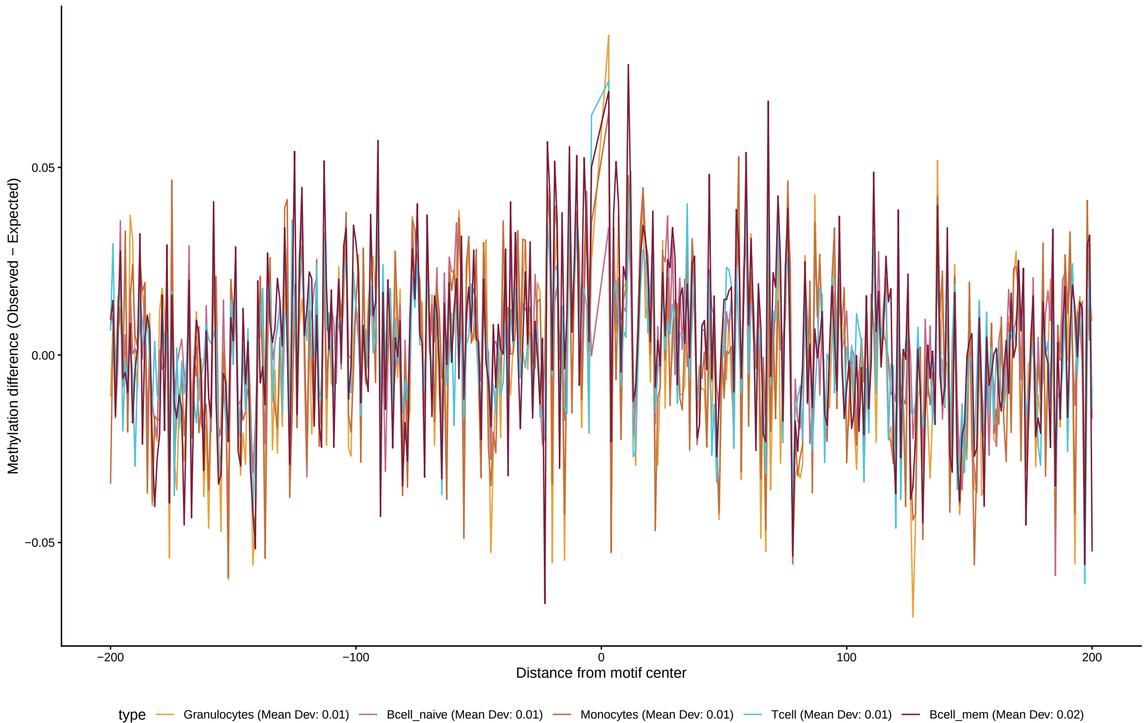
TF footprint difference for TEAD3
