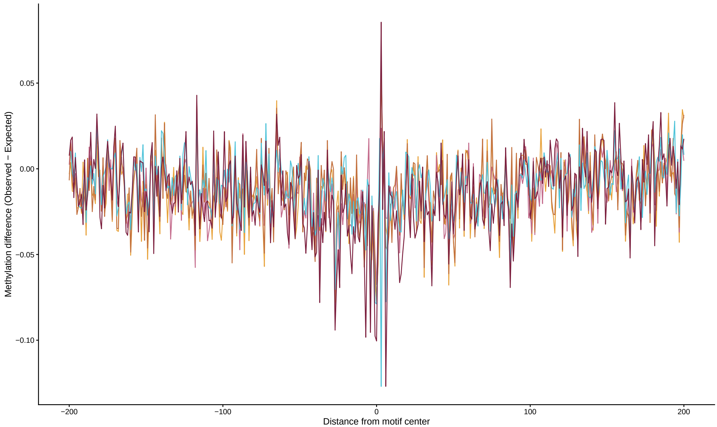
TF footprint difference for TFAP2B
