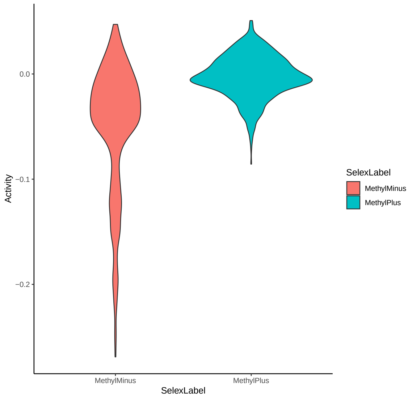
TF activity by SELEX label across NK
