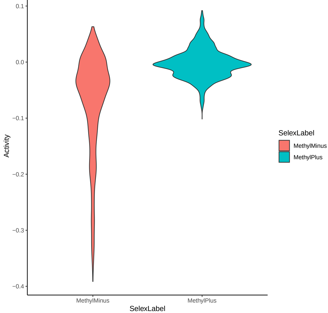
TF activity by SELEX label across gran
