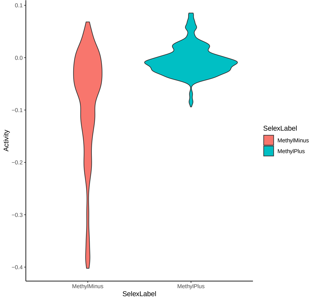
TF activity by SELEX label across mono
