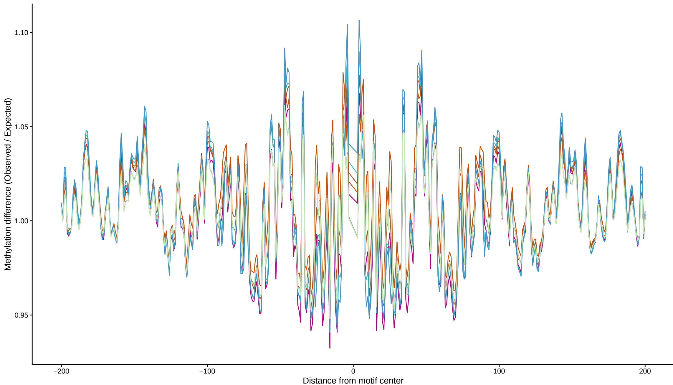
TF footprint difference for ASCL1(var.2)
