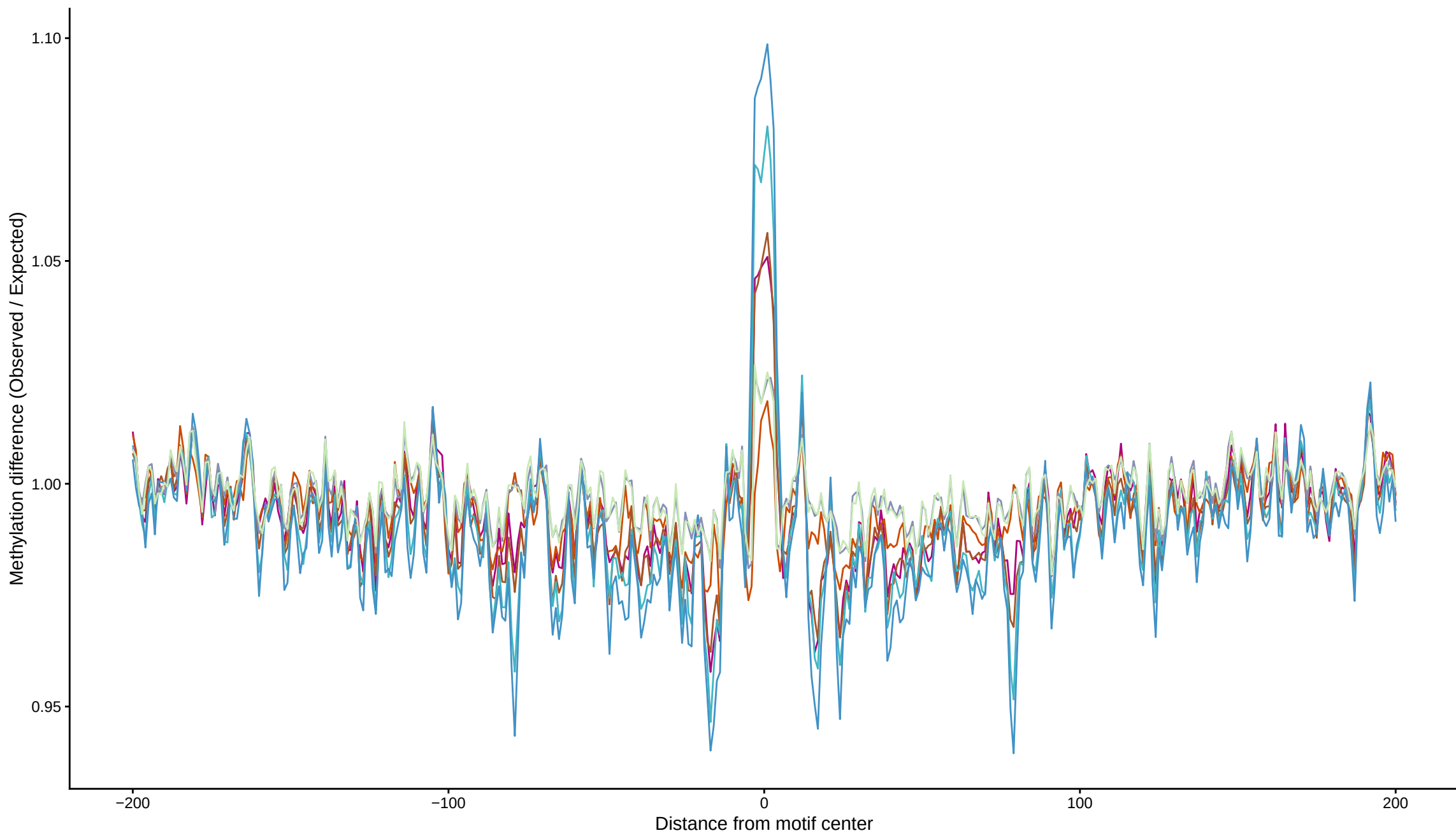
TF footprint difference for TCF21(var.2)
