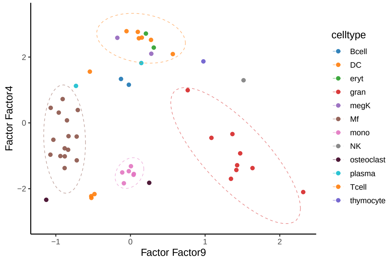
MOFA: Factor Factor9 vs Factor4 (colored by celltype)
