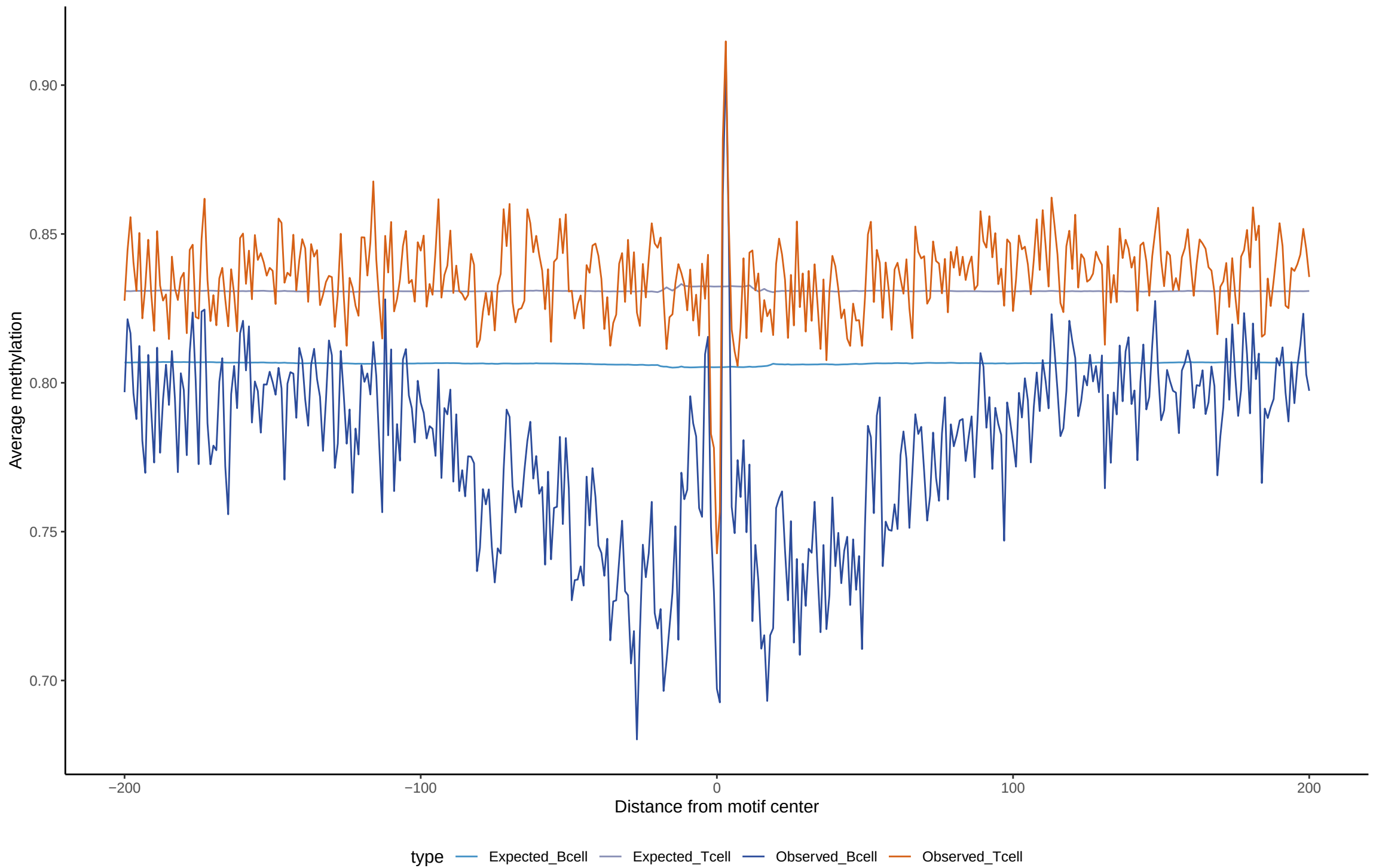
Expected vs observed footprints for EBF3
