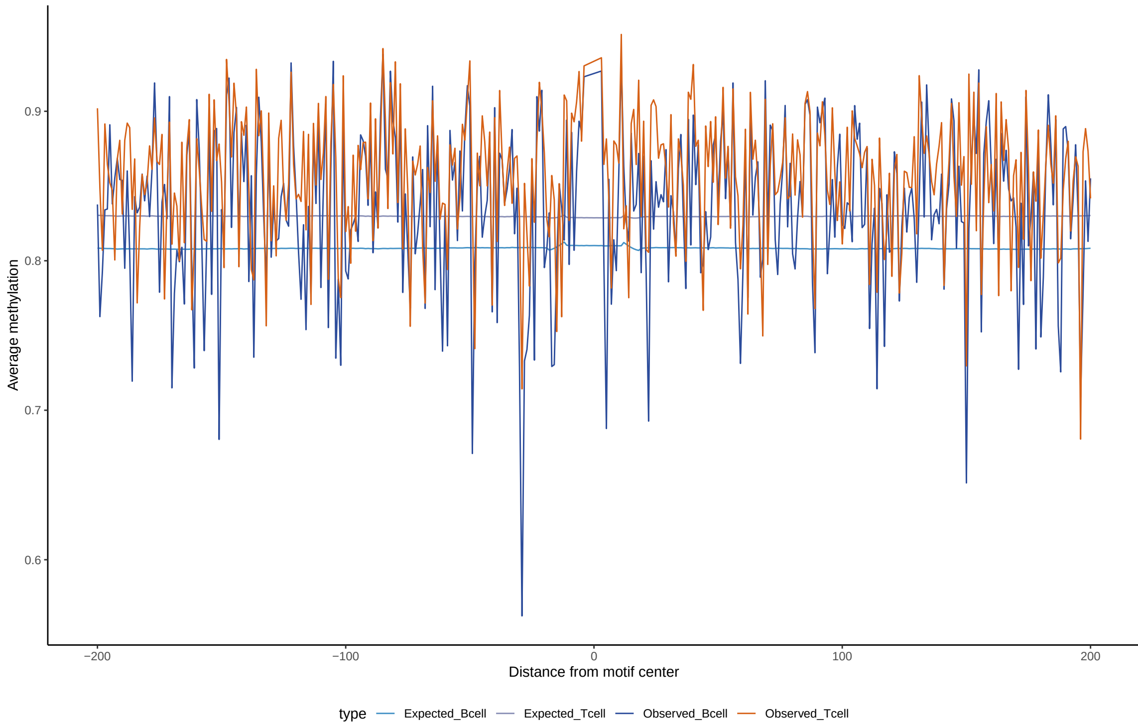
Expected vs observed footprints for EMX1
