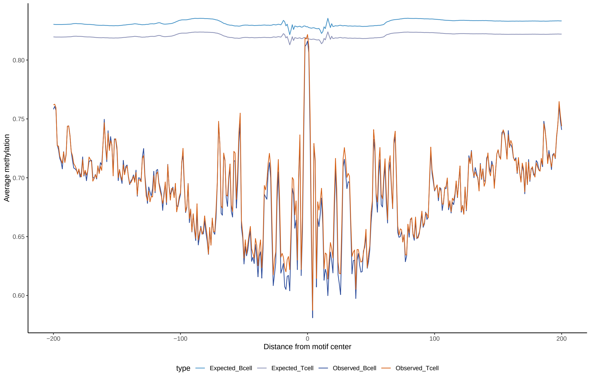
Expected vs observed footprints for ELF4
