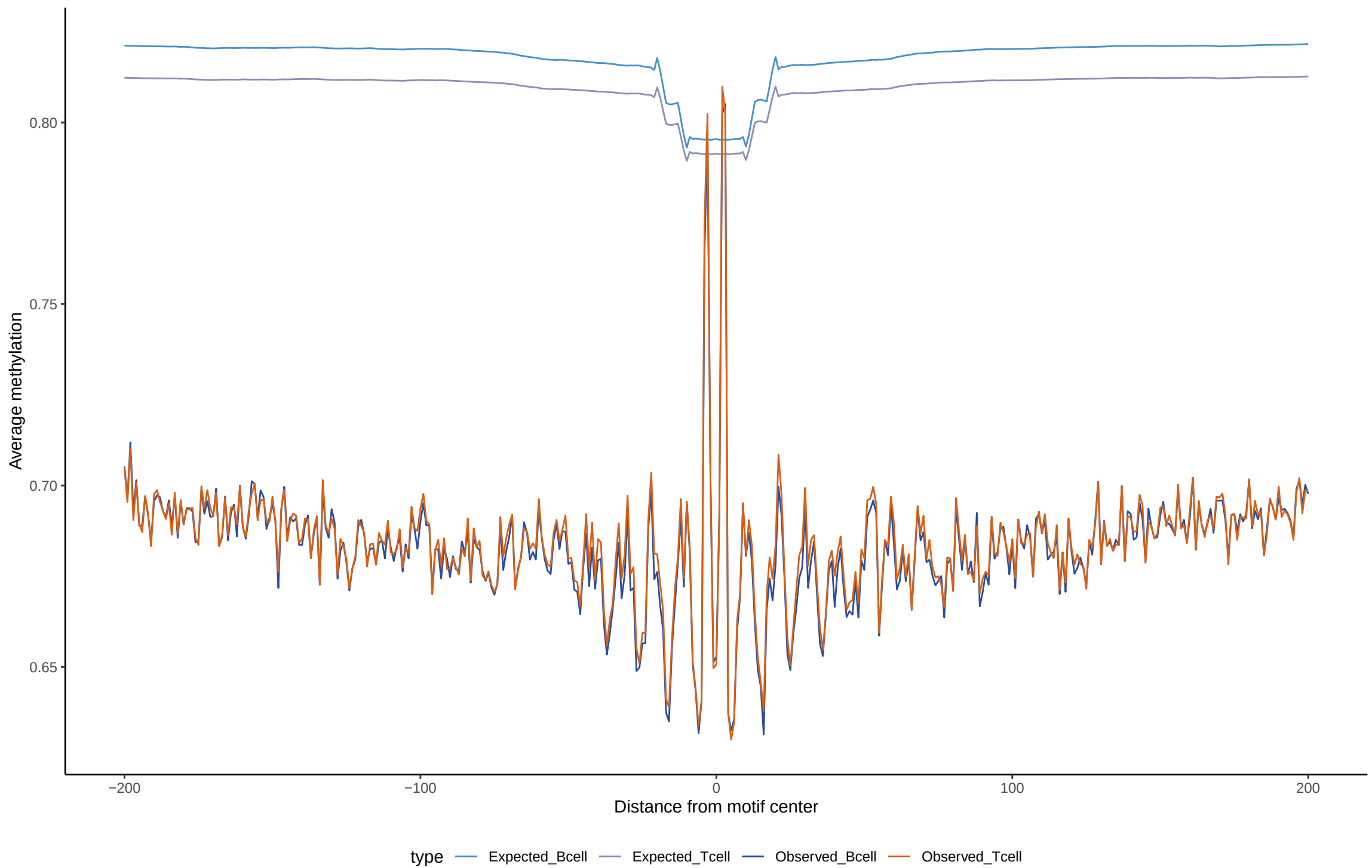
Expected vs observed footprints for TFAP2C
