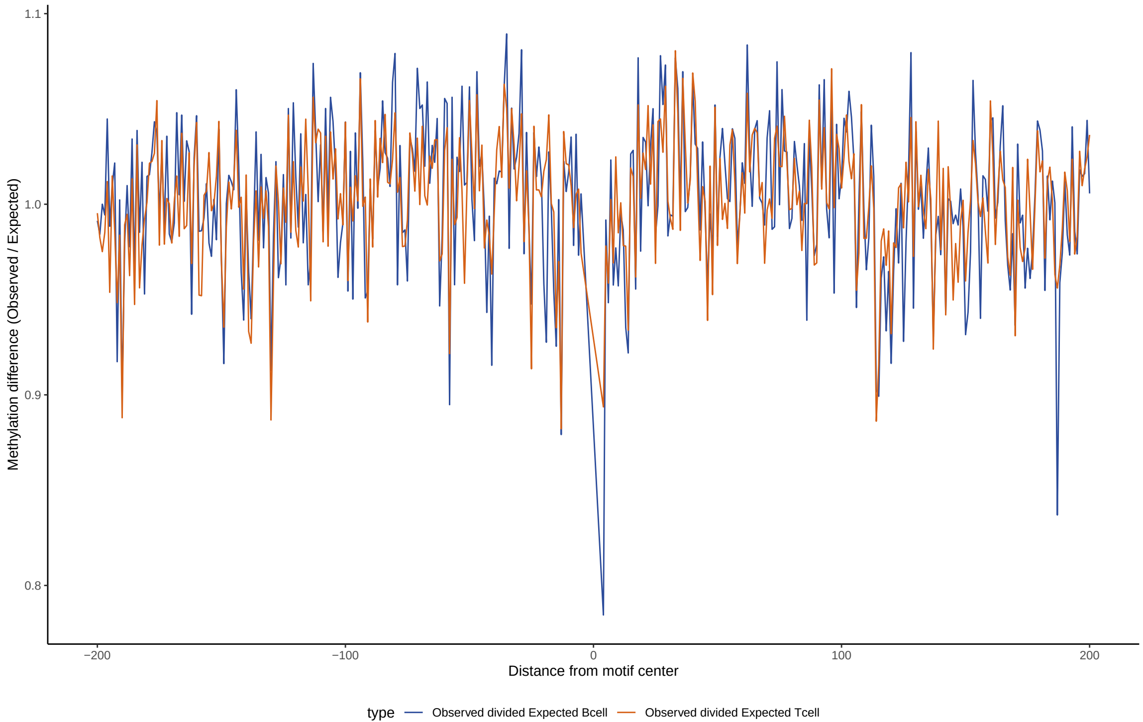
TF footprint difference for ALX3
