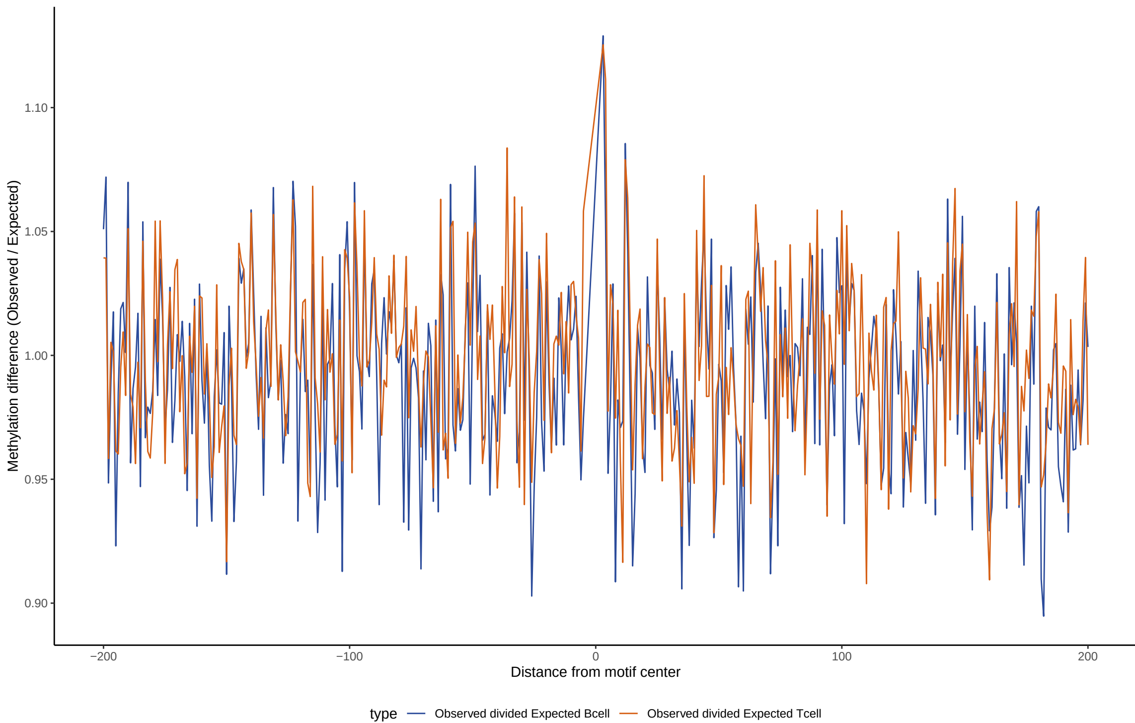
TF footprint difference for BARX1
