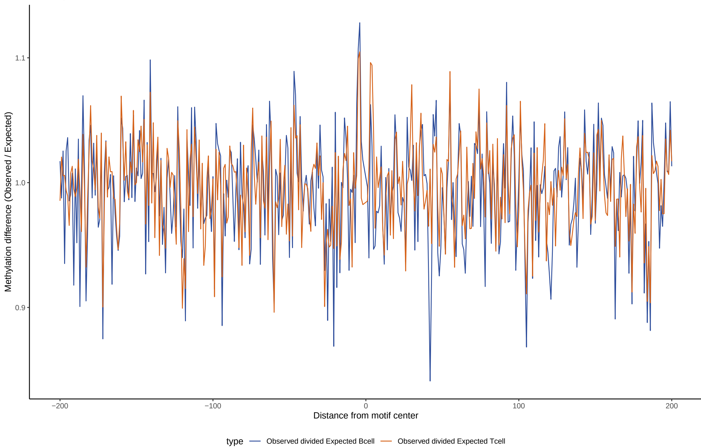
TF footprint difference for BHLHE23
