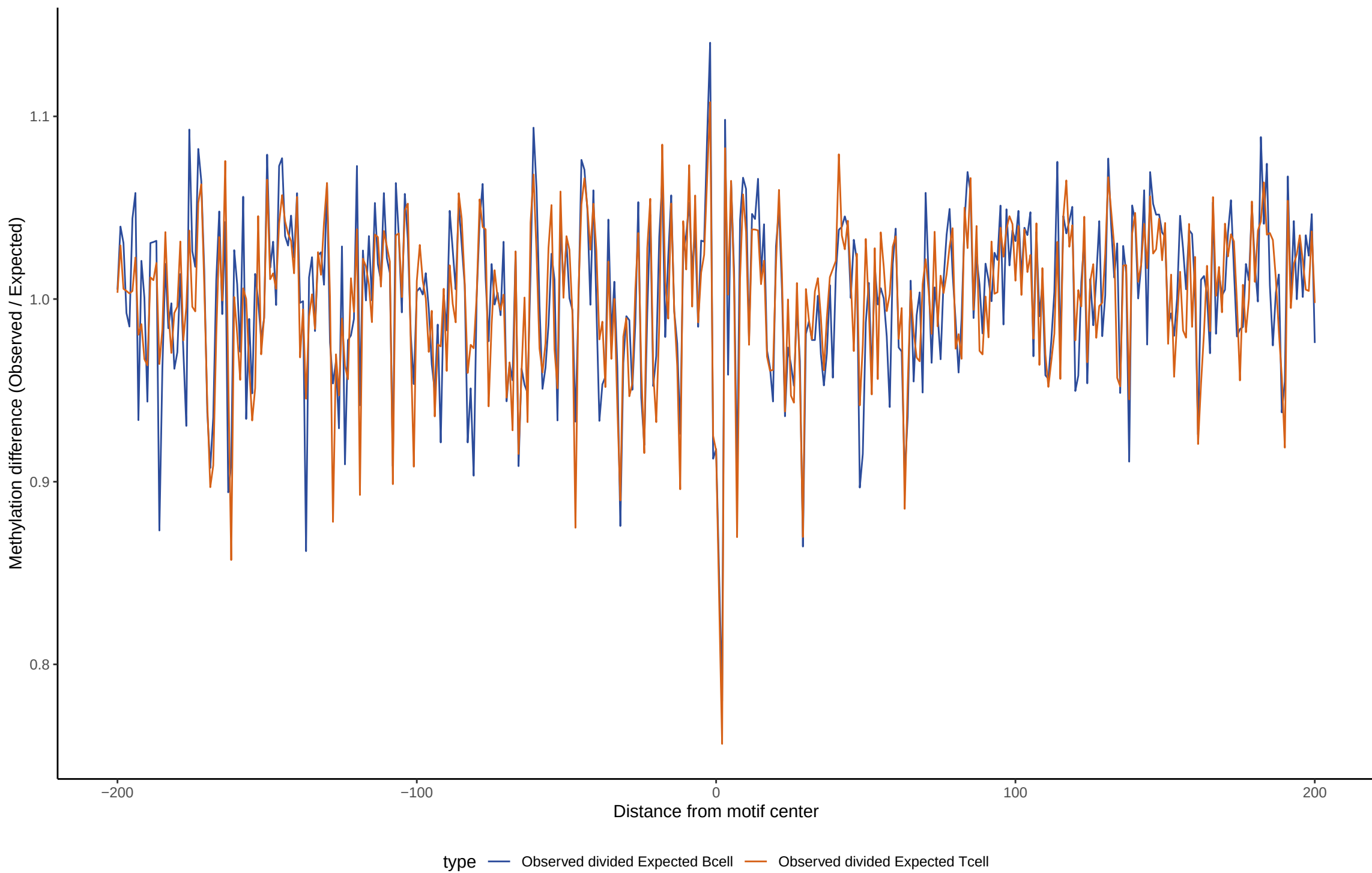
TF footprint difference for BHLHE41
