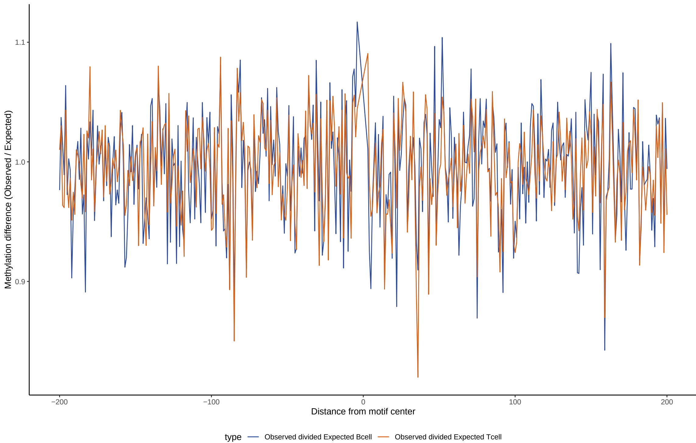
TF footprint difference for BSX
