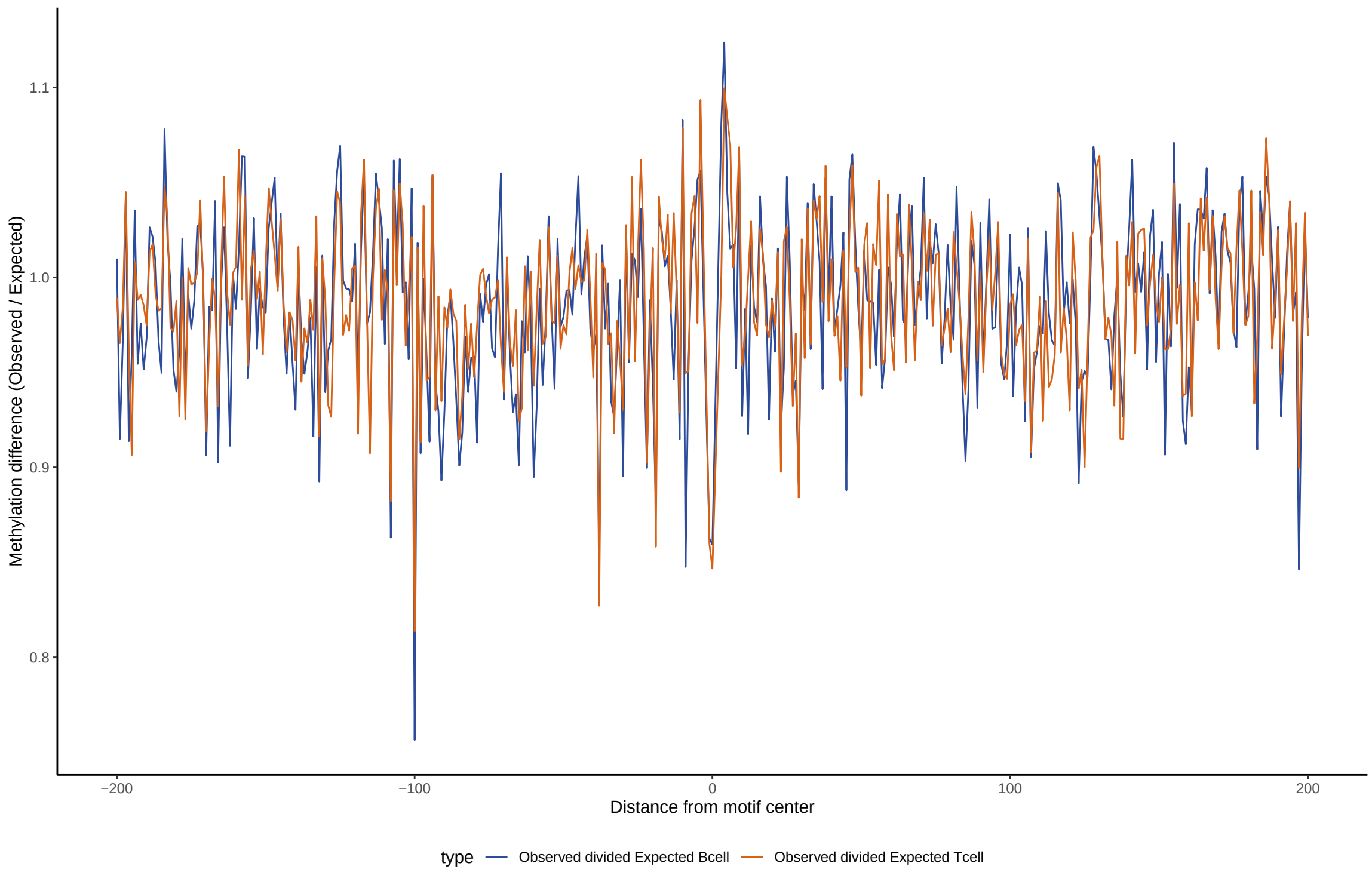
TF footprint difference for CLOCK
