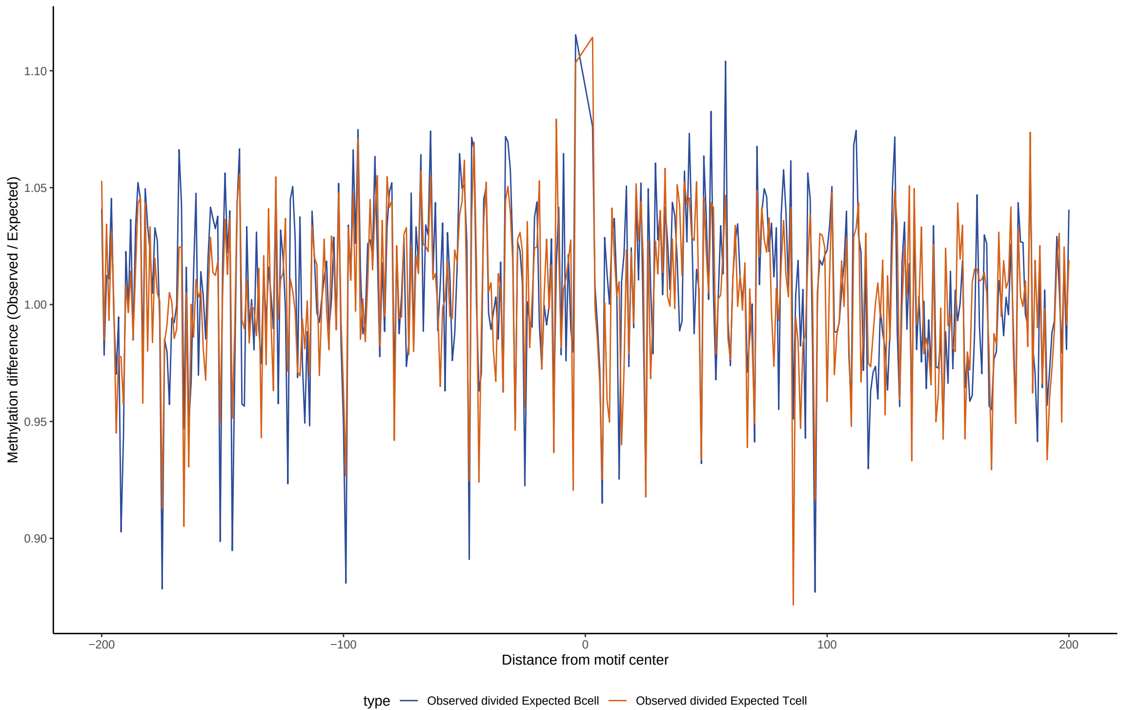
TF footprint difference for DLX6
