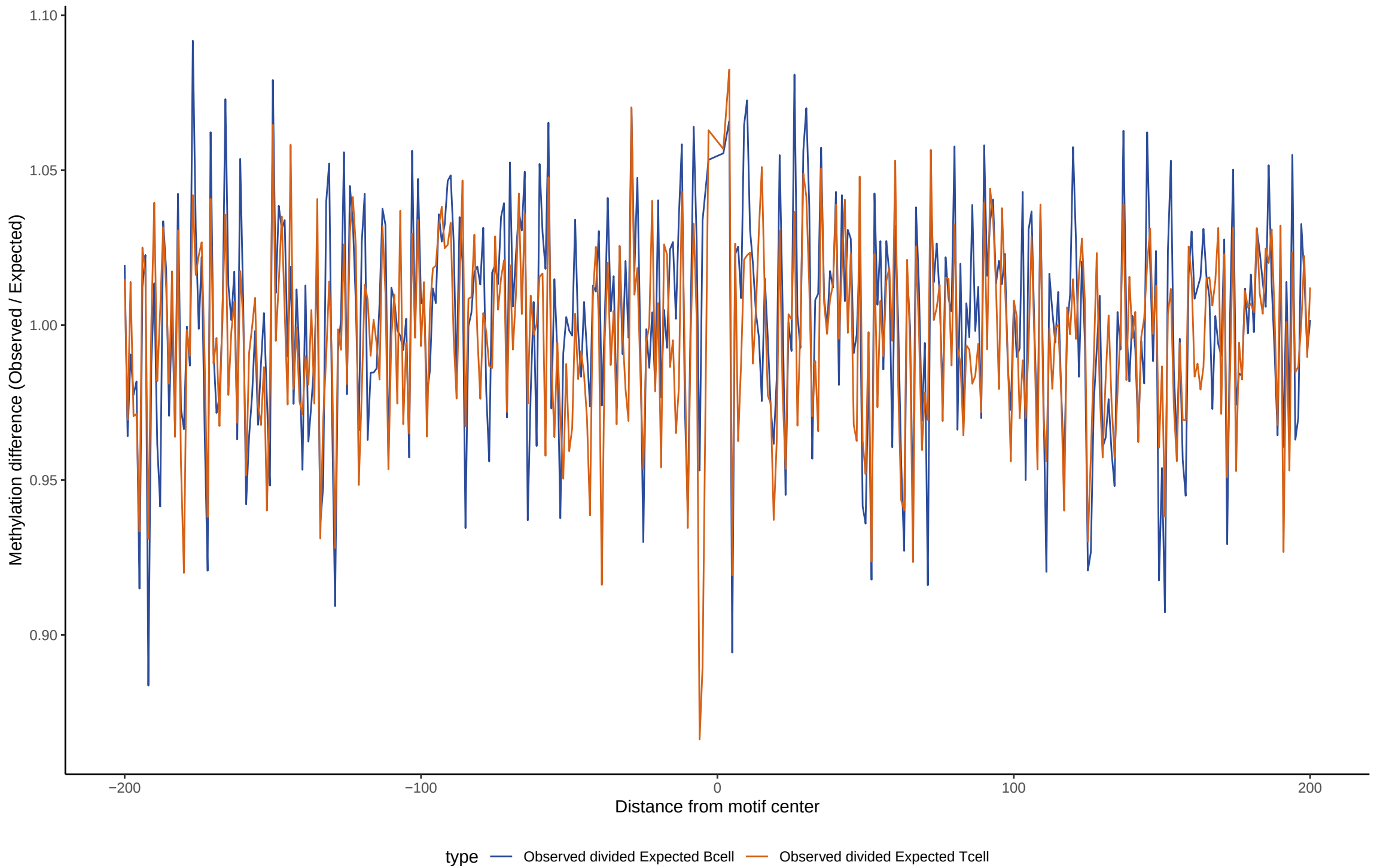
TF footprint difference for DMRT3
