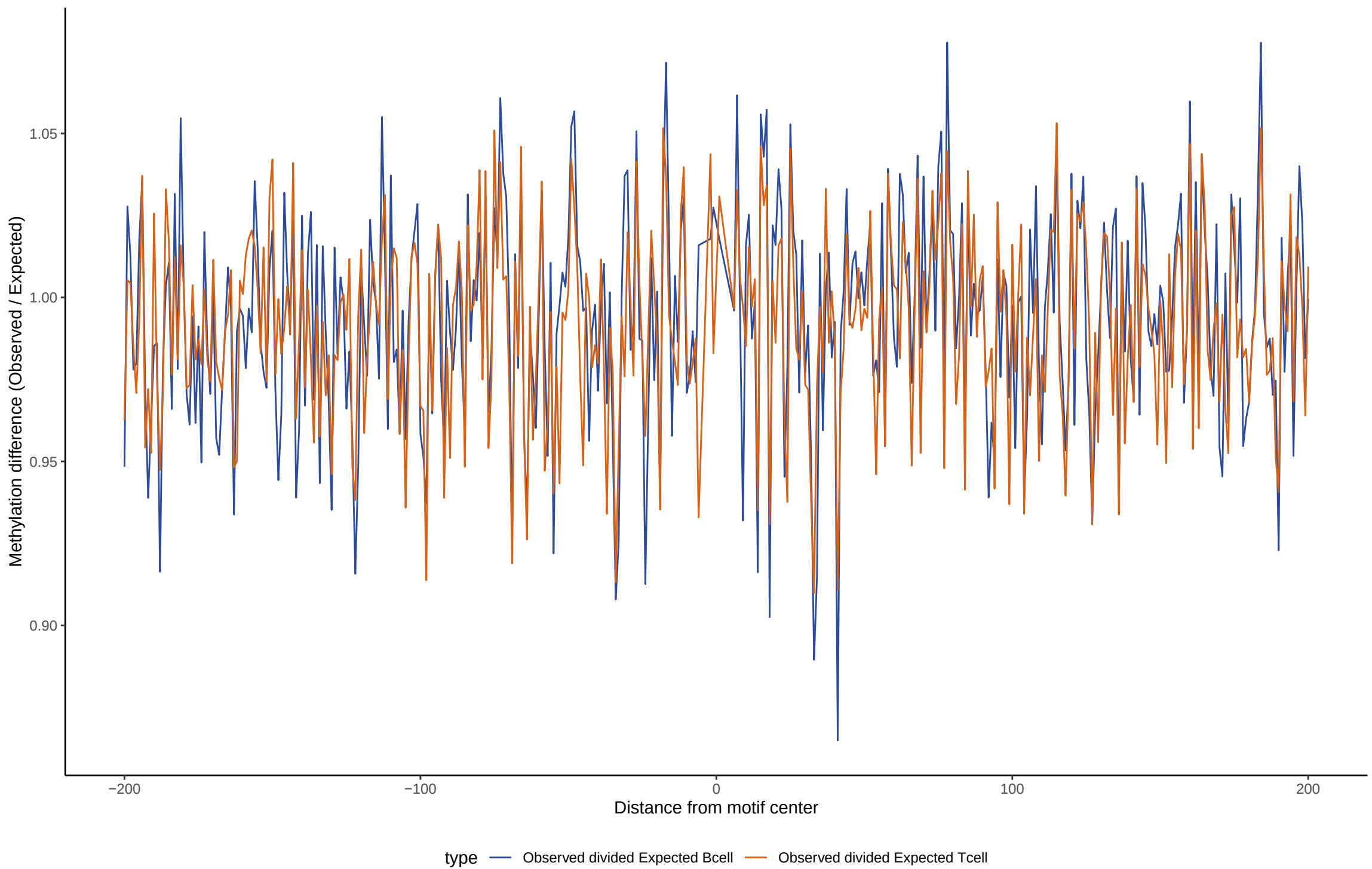
TF footprint difference for DUX4
