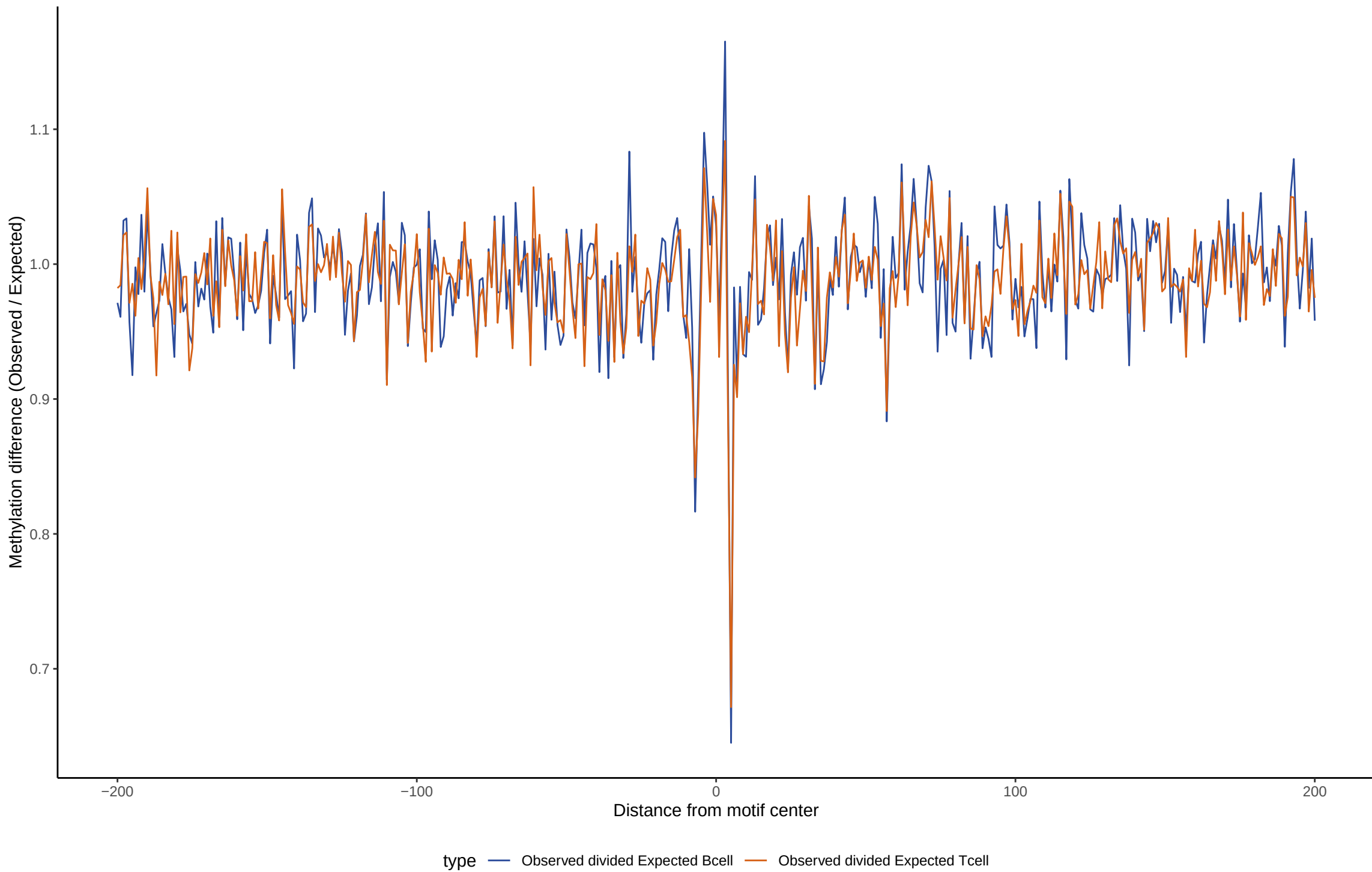
TF footprint difference for E2F7
