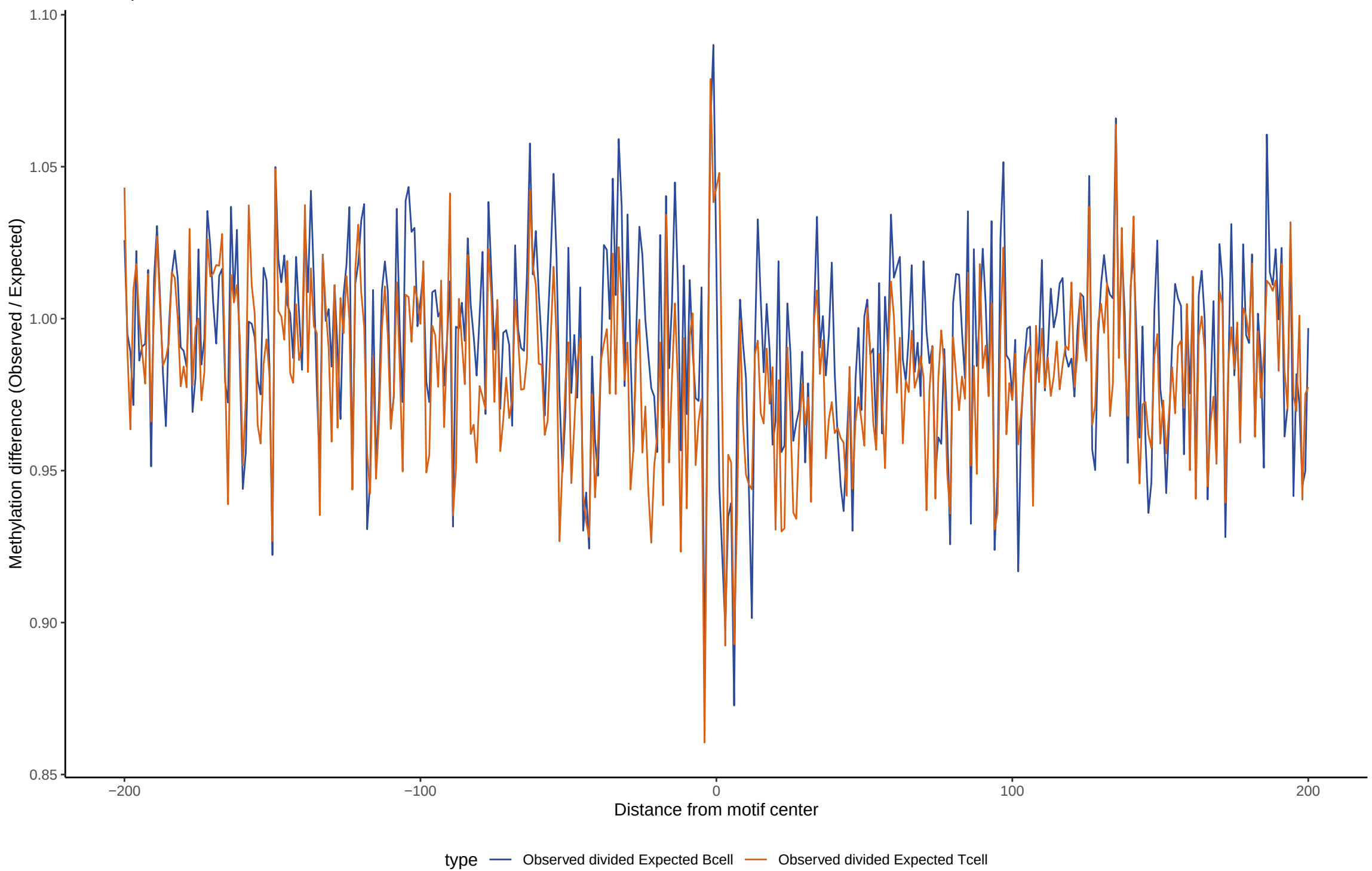
TF footprint difference for EOMES
