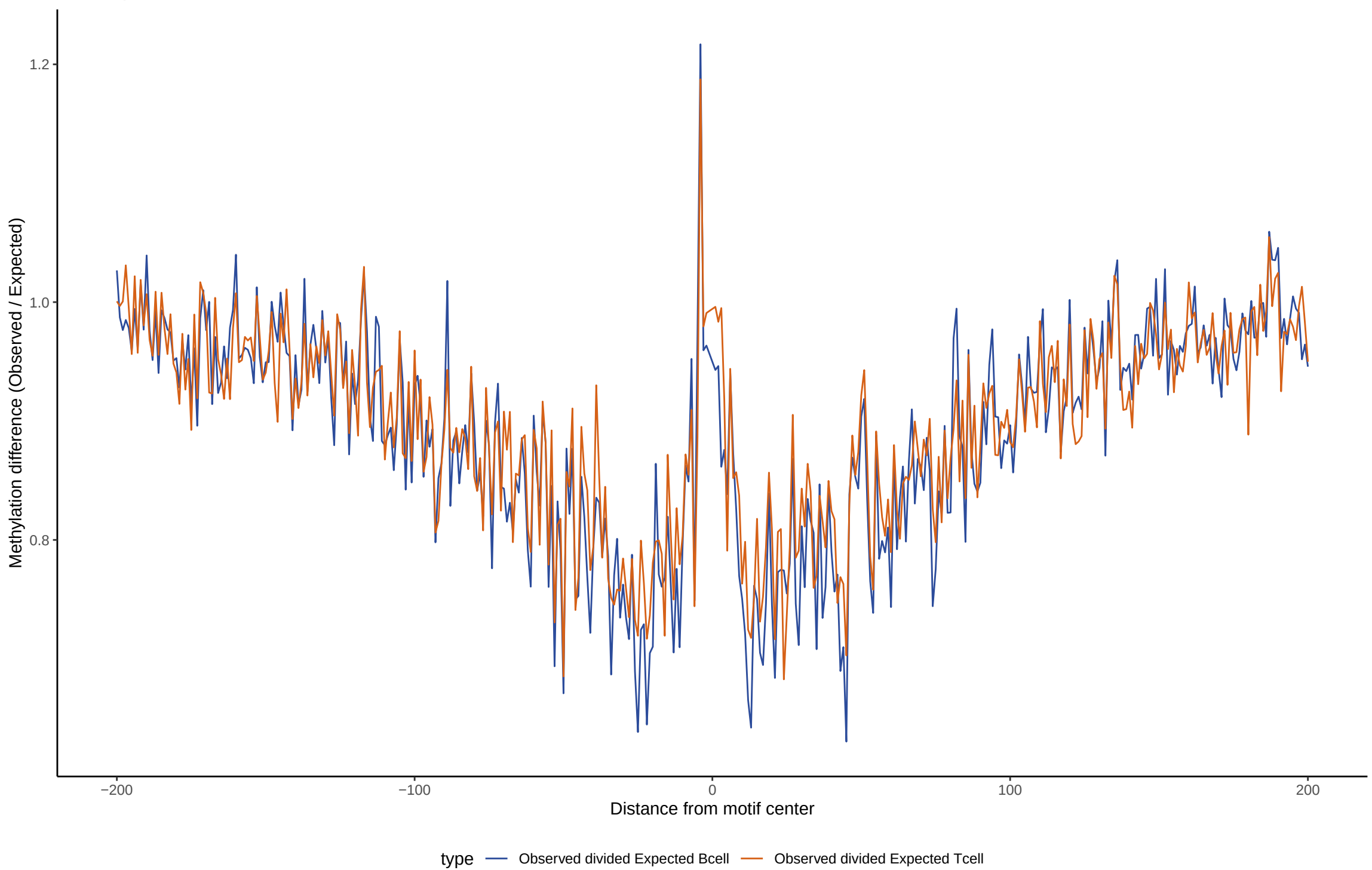
TF footprint difference for ERG
