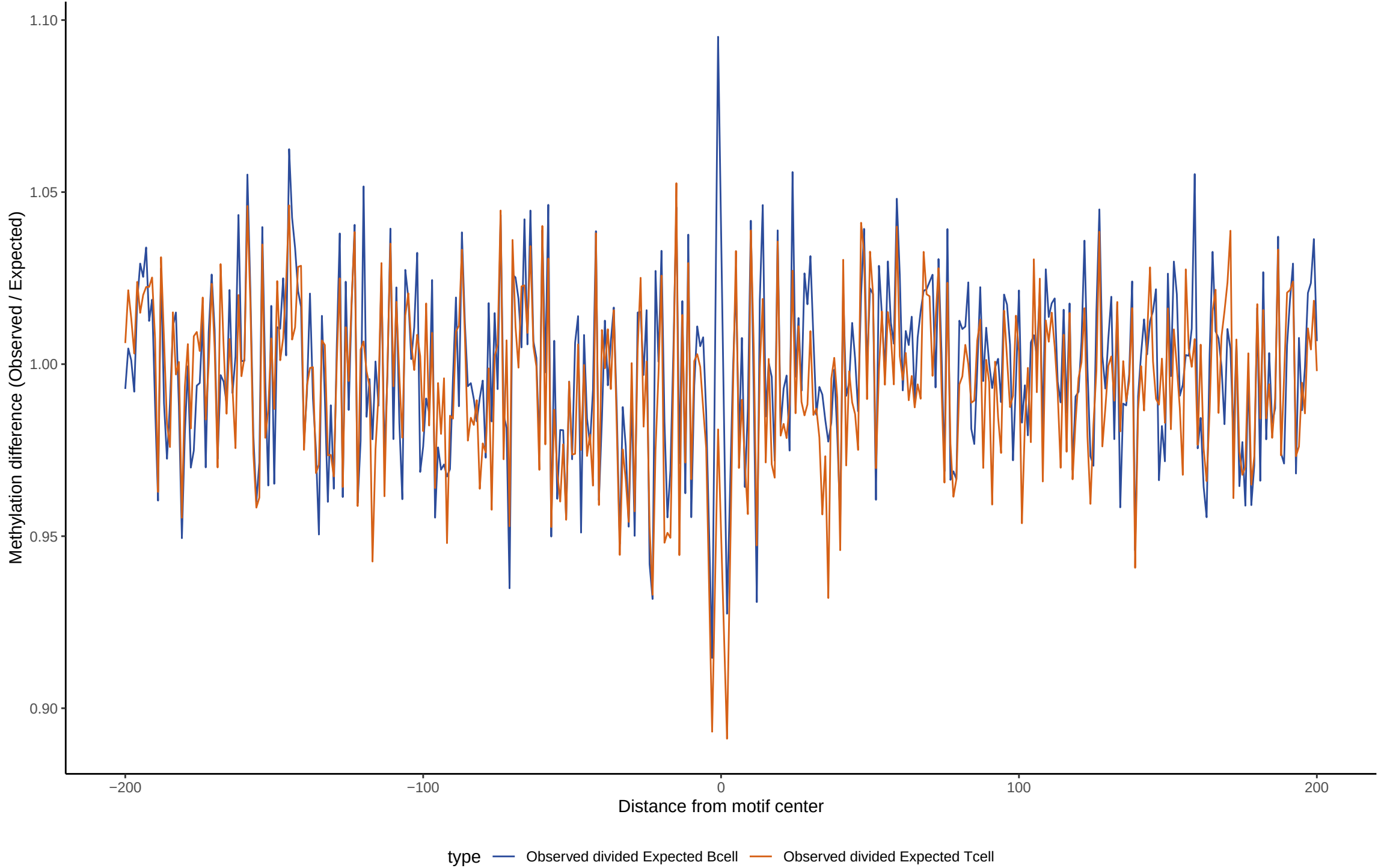
TF footprint difference for ESRRB
