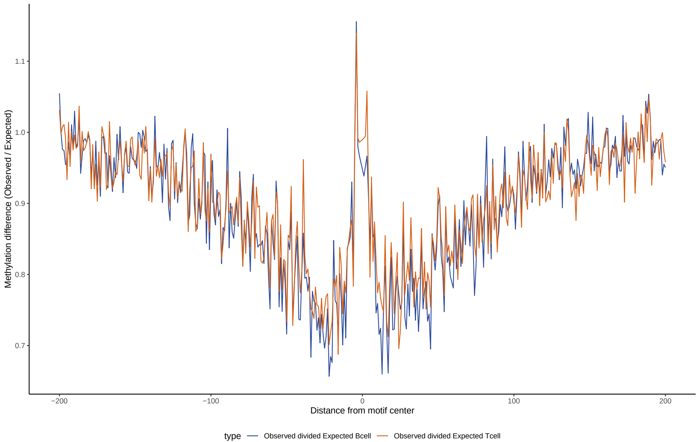
TF footprint difference for ETS1
