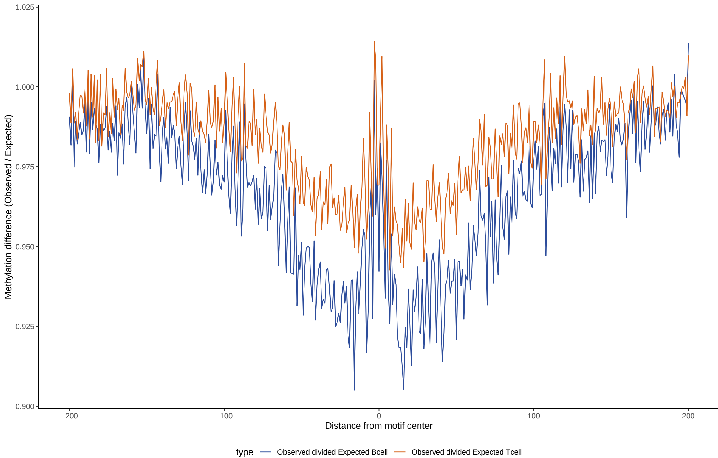
TF footprint difference for EWSR1-FLI1
