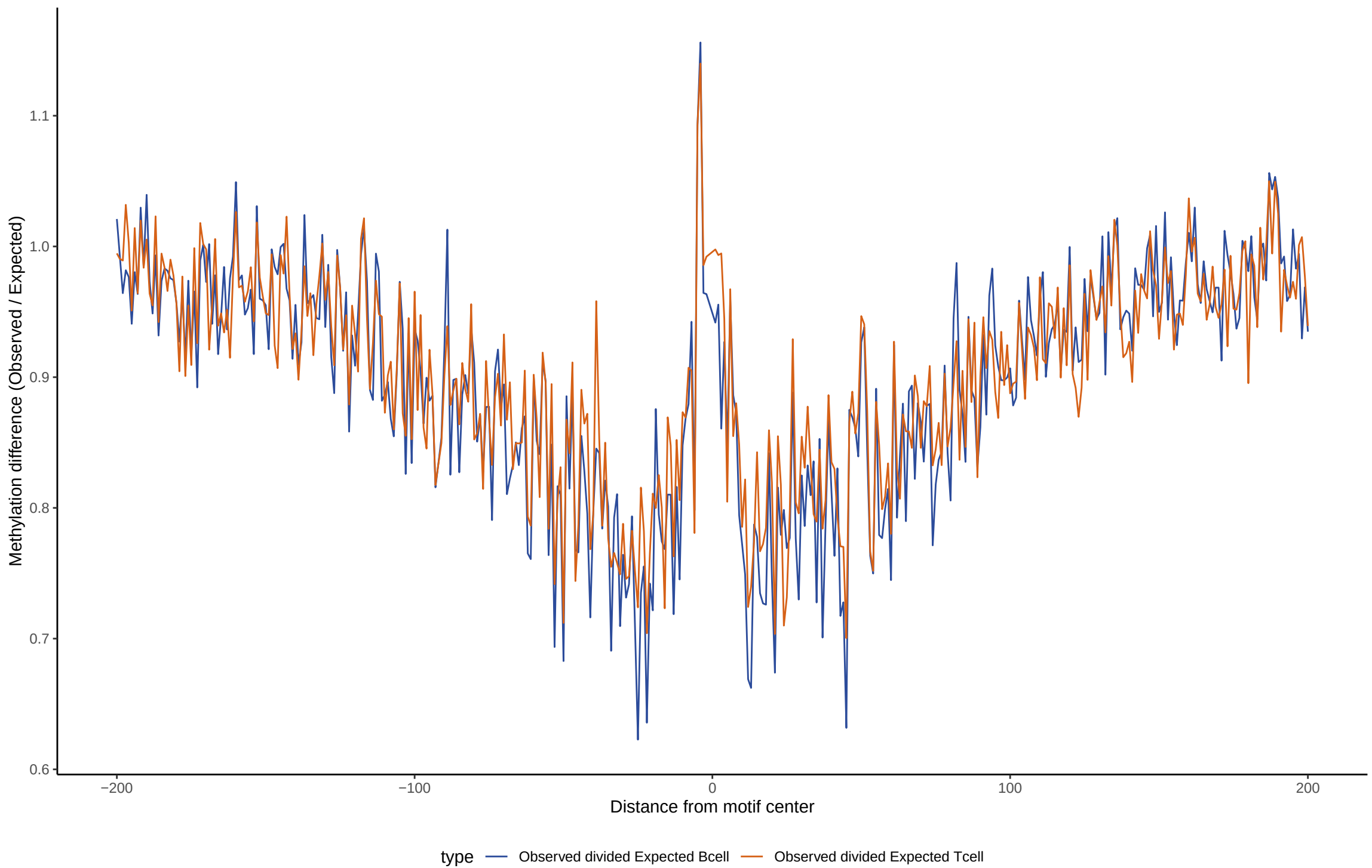
TF footprint difference for FLI1
