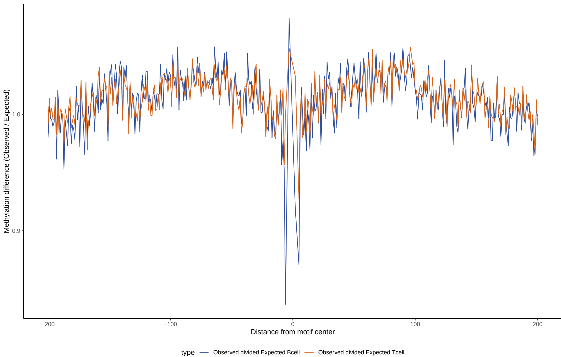
TF footprint difference for FOXB1
