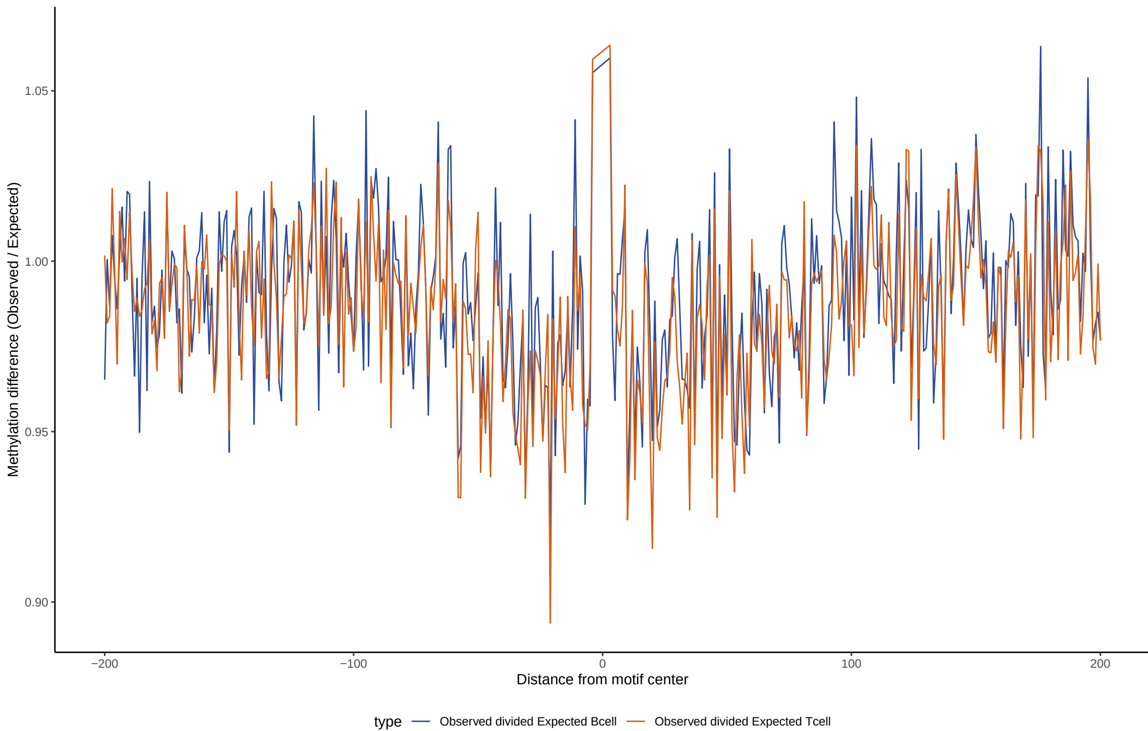
TF footprint difference for FOXI1
