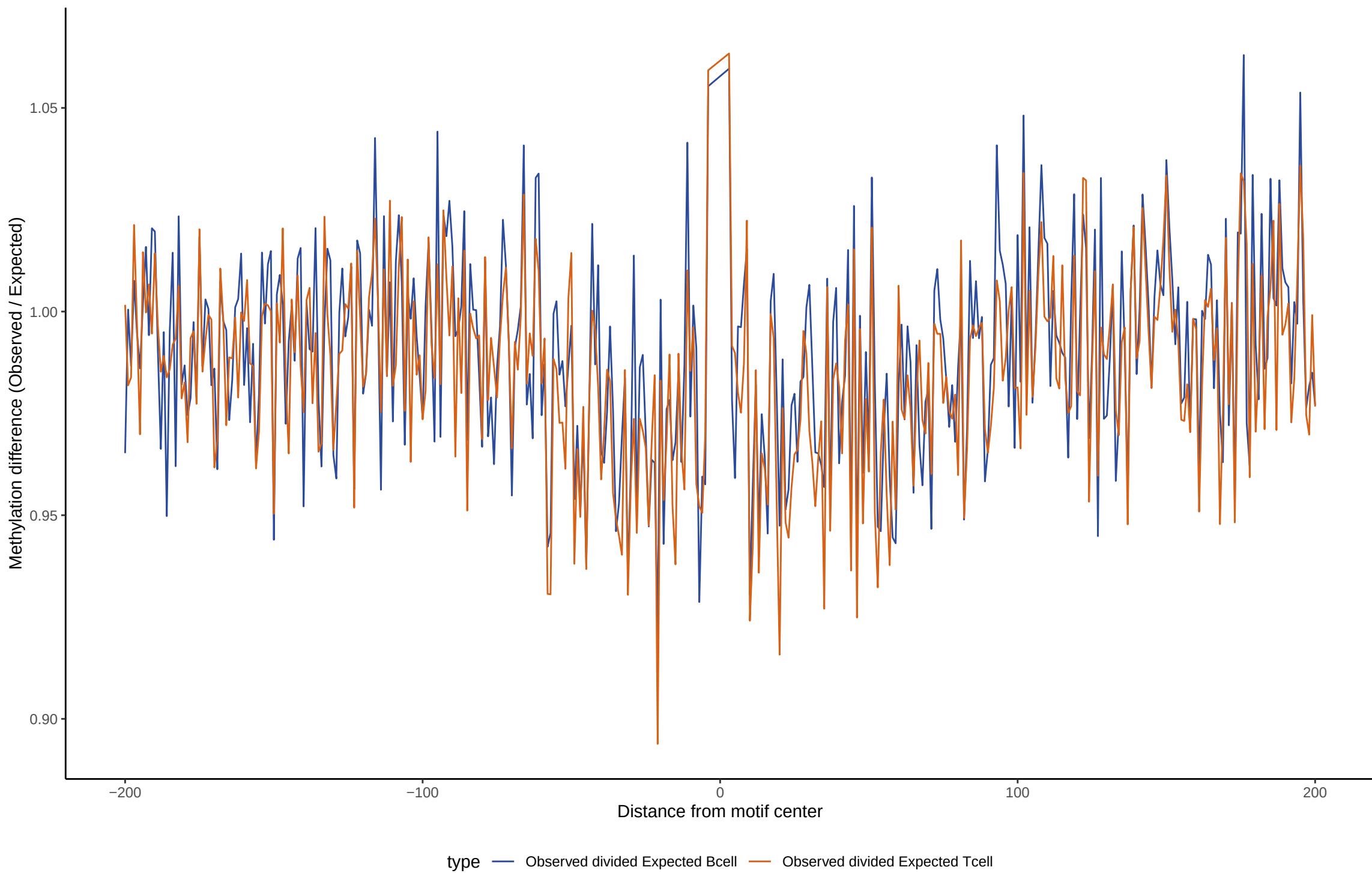
TF footprint difference for FOXO6
