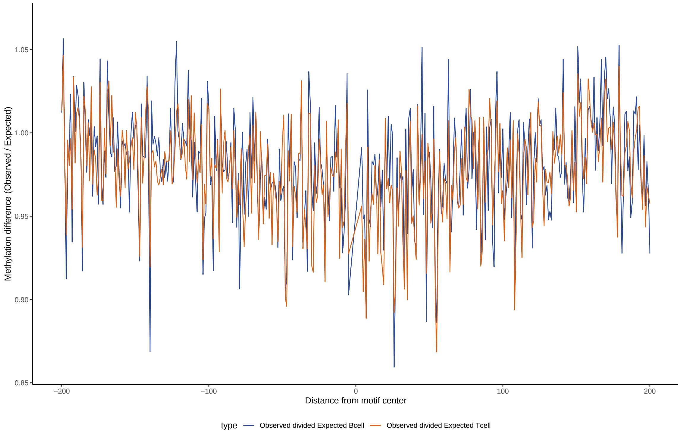
TF footprint difference for GATA2
